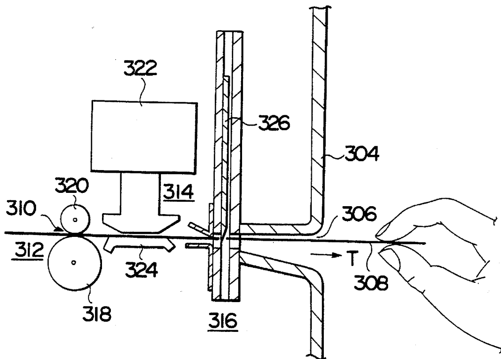
PRIOR ART FIG. 22A
