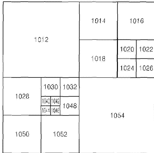
CODING UNIT (1010)
