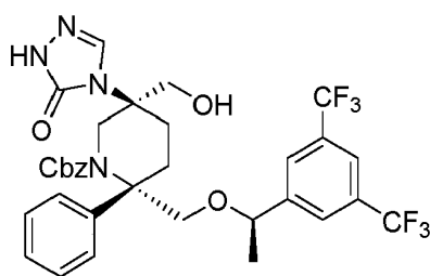
Compound 23h
