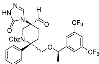
Compound 42f
