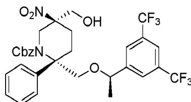
Compound 23c
