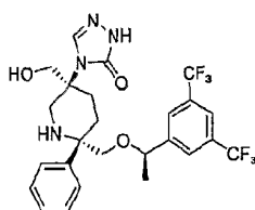
Compound 23
