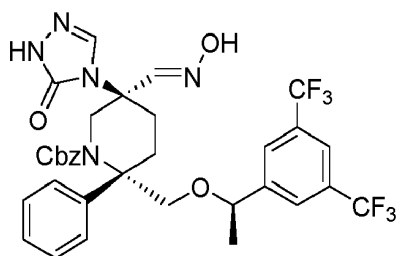
Compound 42g
