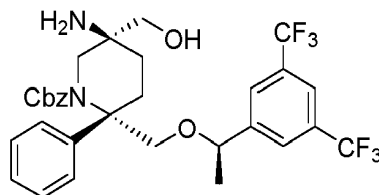
Compound 23e
