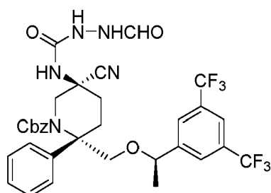
Compound 42d
