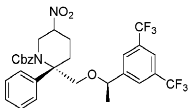
Compound 23b
