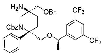
Compound 23f
