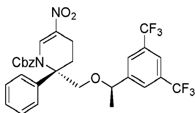
Compound 23a
