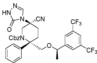
Compound 42i
