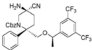
Compound 42b
