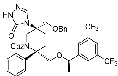
Compound 23g
