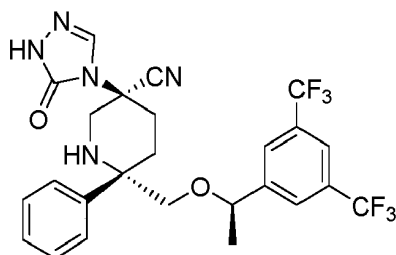
Compound 42
