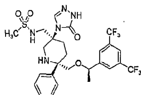
Compound 15
