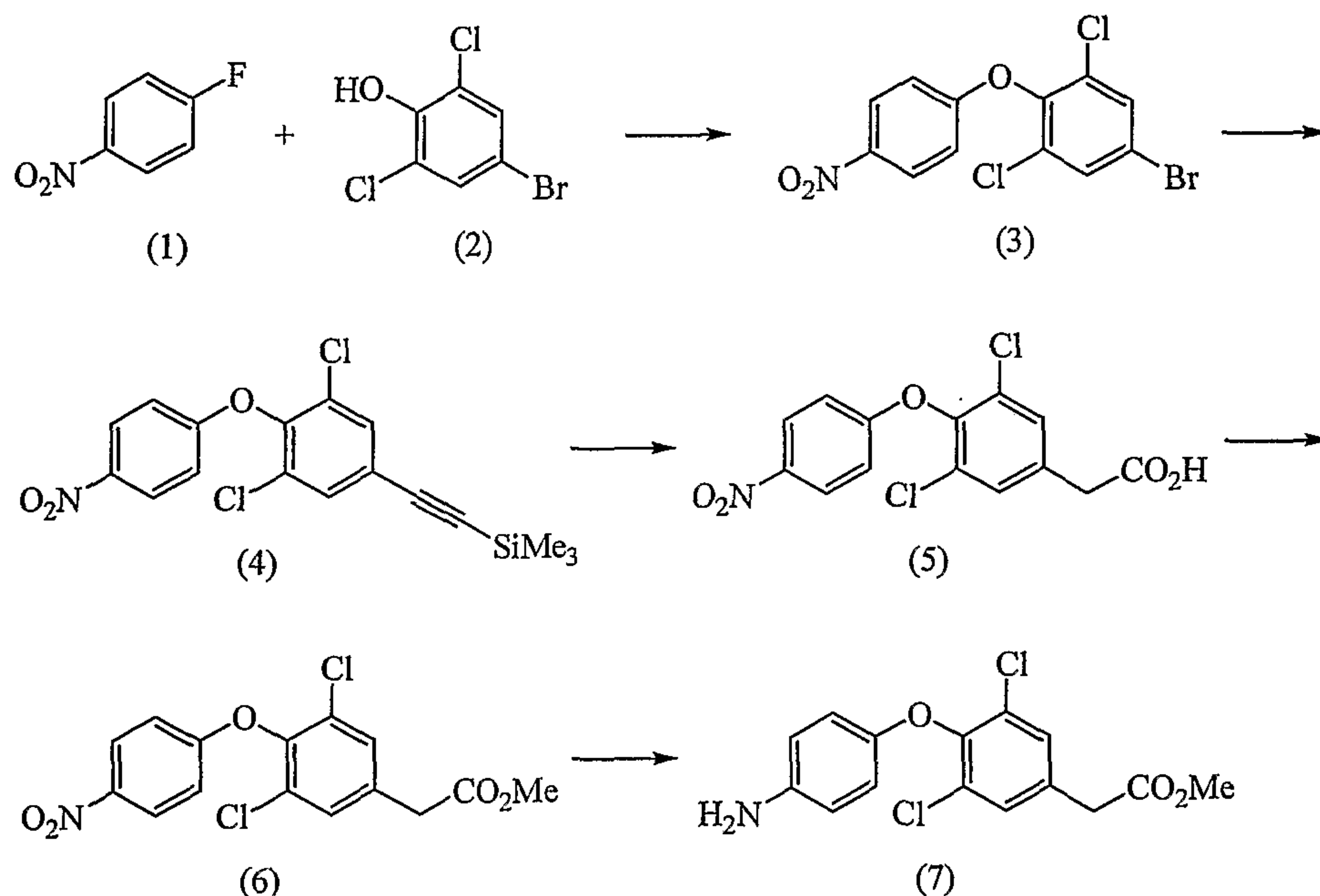
Scheme 1
