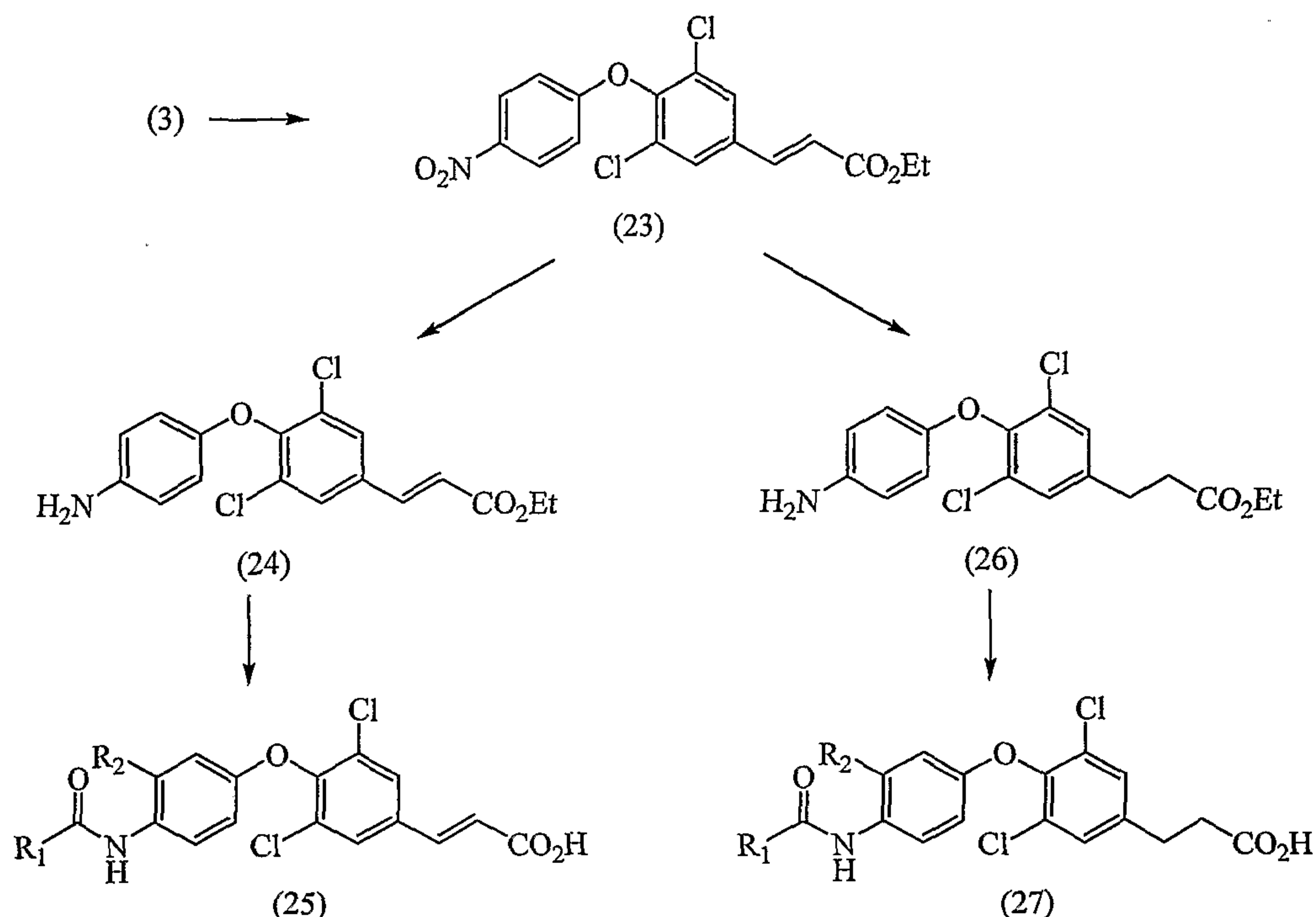
Scheme 8
