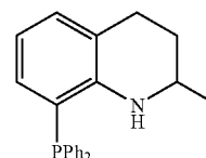
(a) synthesis of 8-Diphenylphosphinoquinoline (1)
