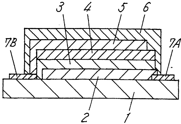
Fig. 16 PRIOR ART
