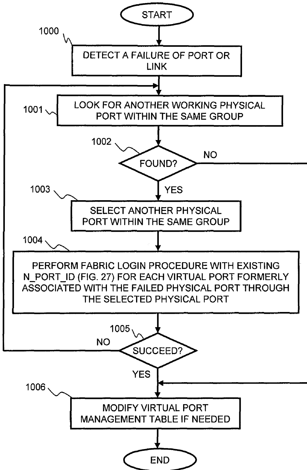
FIG. 10 Flowchart of Port Failover
