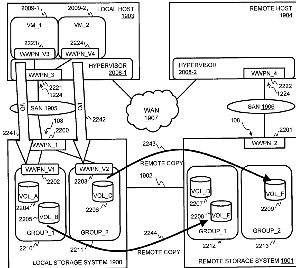
FIG. 22 Conceptual Diagram of 3 rd Embodiment
