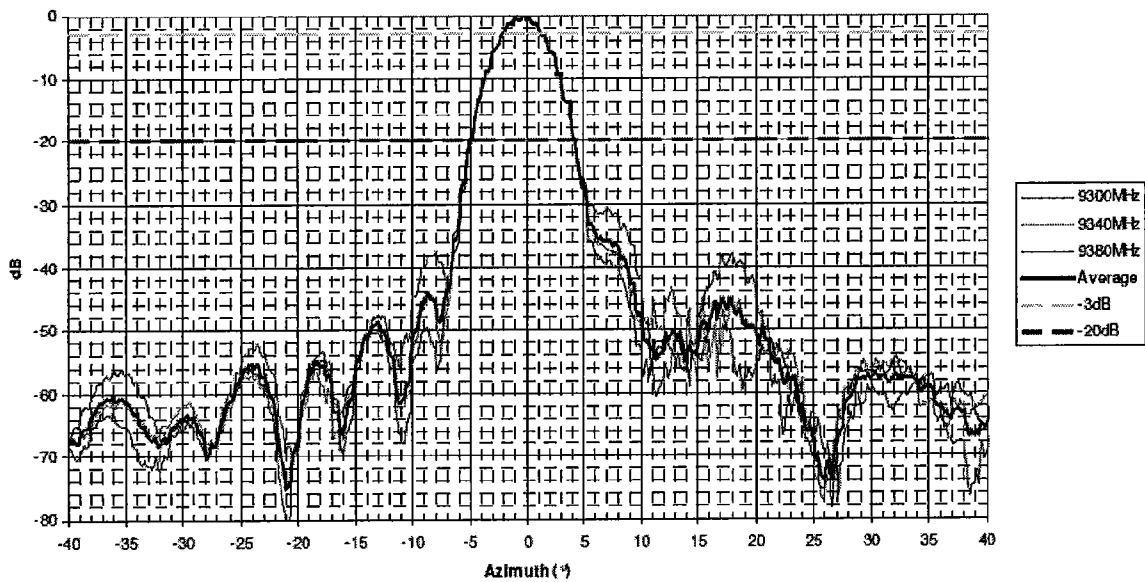
Measured Two Way BR24 Antenna Azimuth Response
