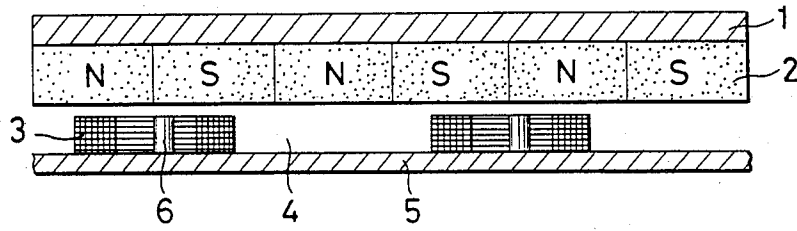
FIG. 2- PRIOR ART
