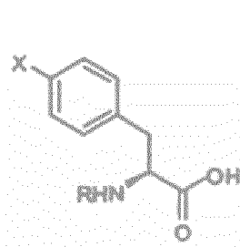
Formel (I)
