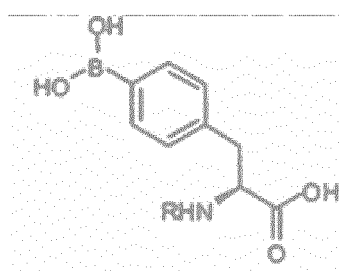
Formel (II)
