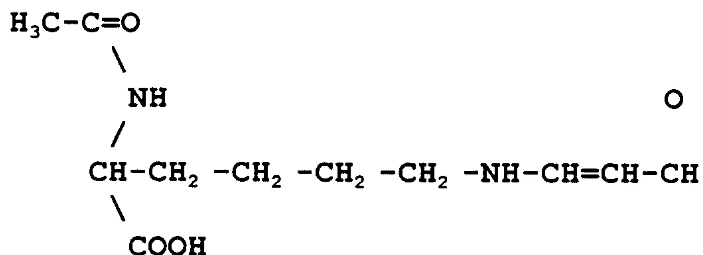
N-alpha-acetyl-epsilon-(2-propenal) lysine
