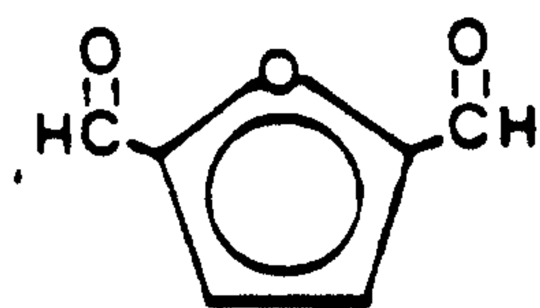
2,5-furandialdehyde
