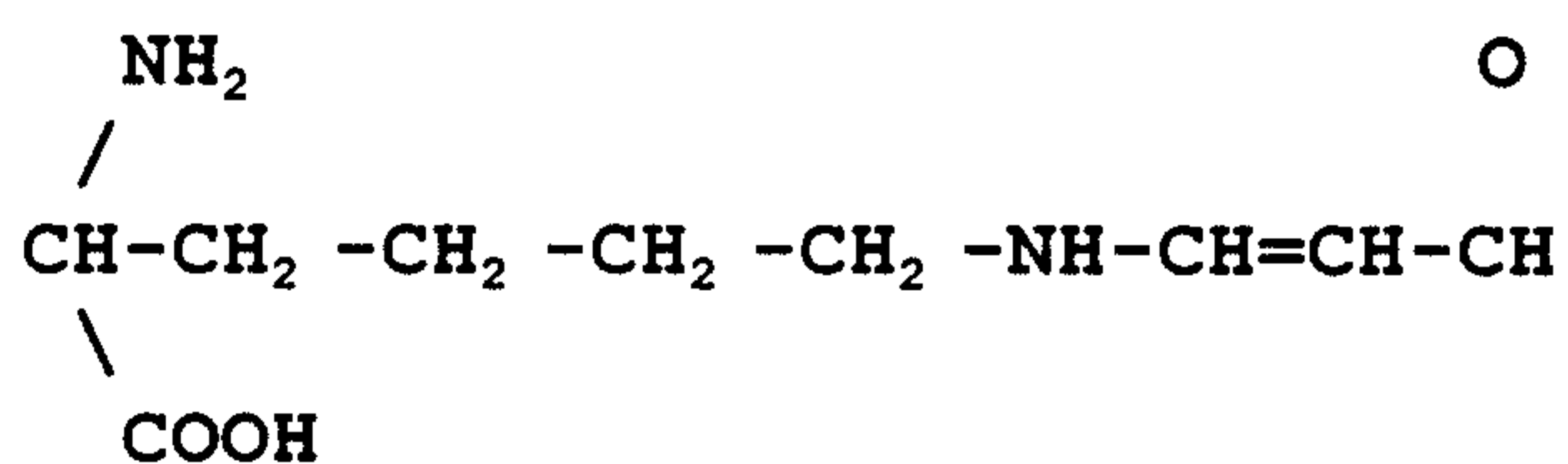
N-epsilon-(2-propenal) lysine
