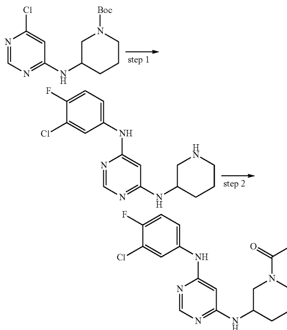
Synthesis of 1-(3-(6-(3-chloro-4-fluorophenylamino)pyrimidin-4-ylamino)piperidin-1-yl)prop-2-en-1-one (I-71)
