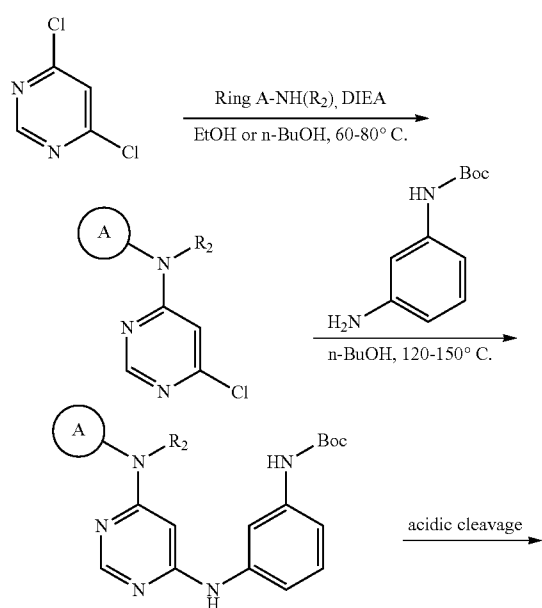
SCHEME 2b Sequence B for Synthesis of 3-(6-mono- or disubstituted-aminopyrimidin-4-yl)amino-phenylamines
