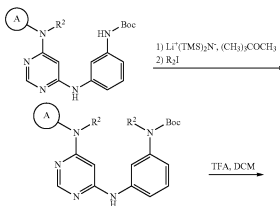
SCHEME 2c Synthesis of 3-(6-mono or disubstituted-aminopyrimidin-4-yl)amino-N-substituted phenylamines
