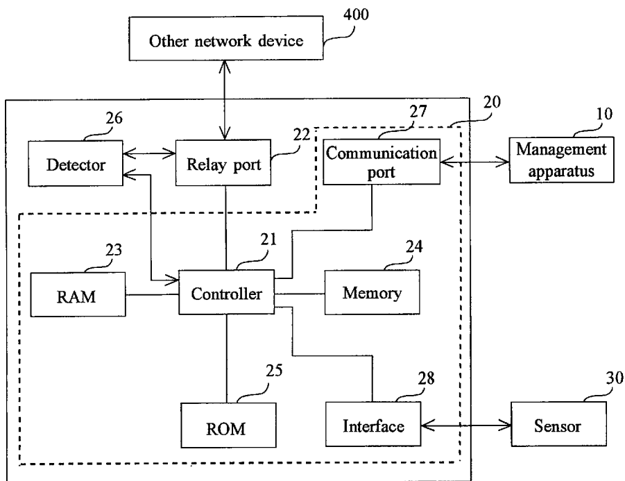
Network device 40 having sensor control apparatus 20
