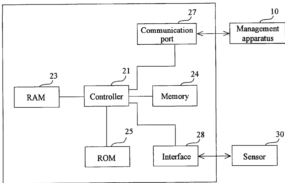
Sensor controller 20 (Terminal device)
