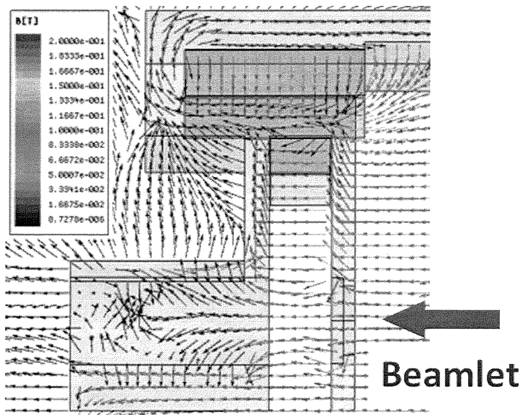
Magnetic field distribution within a depressed collector
