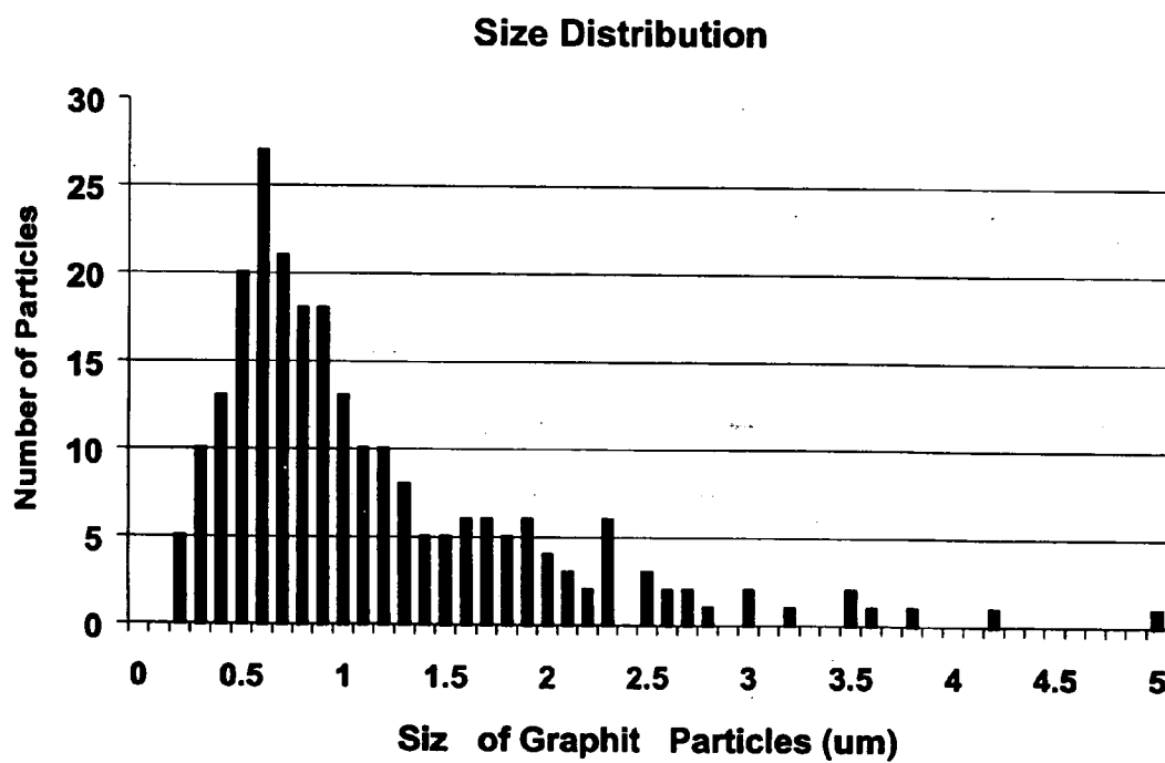
FIG. 6 Size Distribution of Exfoliated Graphite Platelets
