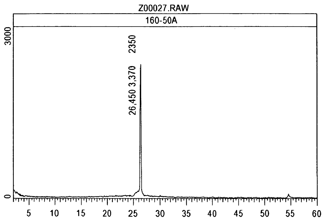
FIG. 3 X-Ray Diffraction Pattern of Intercalated Natural Graphite
