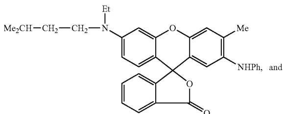
2-Anilino-3-methyl-6-(di-n-amylamino)fluoran
