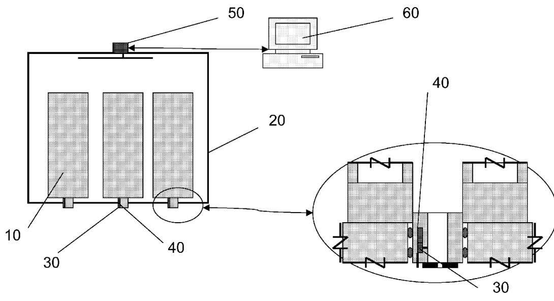
Figure 3: In- Situ Integrity Test Configuration Transmembrane Pressure Probe / RFID Communication Device within Multi-Element Filter Configuration
