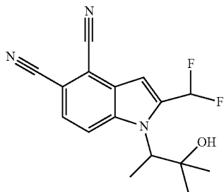
B. 2-(Difluoromethyl)-1-(3-hydroxy-3-methylbutan-2-yl)-1H-indole-4,5-dicarbonitrile
