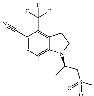
(R)-1-(1-(Methylsulfonyl)propan-2-yl)-4-(trifluoromethyl)indoline-5-carbonitrile
