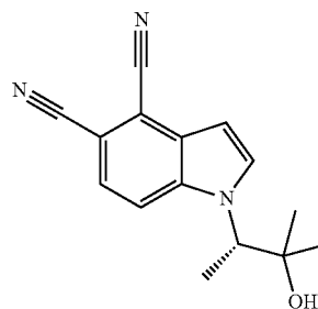
(S)-1-(3-Hydroxy-3-methylbutan-2-yl)-1H-indole-4,5-dicarbonitrile
