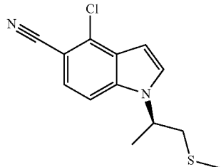
(R)-4-Chloro-1-(1-(methylthio)propan-2-yl)-1H-indole-5-carbonitrile
