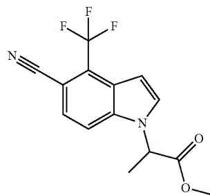
A. Methyl 2-(5-cyano-4-(trifluoromethyl)-1H-indol-1-yl)propanoate
