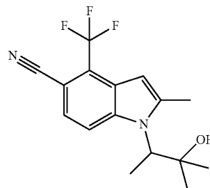
2-Methyl-1-(1-methyl-2-oxopropyl)-4-(trifluoromethyl)-1H-indole-5-carbonitrile (Ex. 3) and 1-(2-Hydroxy-1,2-dimethylpropyl)-2-methyl-4-(trifluoromethyl)-1H-indole-5-carbonitrile (Ex. 4)
