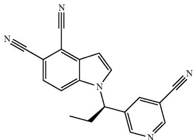
B. (R)-1-(1-(5-Cyanopyridin-3-yl)propyl)-1H-indole-4,5-dicarbonitrile
