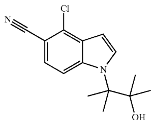
B. 4-Chloro-1-(3-hydroxy-2,3-dimethylbutan-2-yl)-1H-indole-5-carbonitrile
