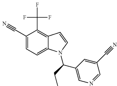
(R)-1-(1-(5-Cyanopyridin-3-yl)propyl)-4-(trifluoromethyl)-1H-indole-5-carbonitrile
