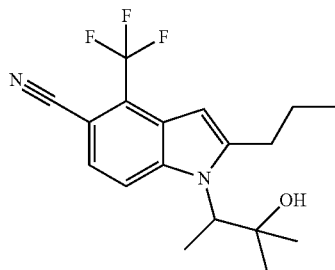
B. 1-(3-Hydroxy-3-methylbutan-2-yl)-2-propyl-4-(trifluoromethyl)-1H-indole-5-carbonitrile
