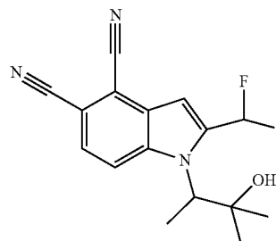
2-(Difluoromethyl)-1-(3-hydroxy-3-methylbutan-2-yl)-1H-indole-4,5-dicarbonitrile
