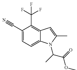
Methyl 2-[5-cyano-2-methyl-4-(trifluoromethyl)-1H-indol-1-yl]propanoate
