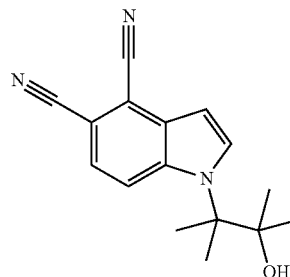
1-(3-Hydroxy-2,3-dimethylbutan-2-yl)-1H-indole-4,5-dicarbonitrile
