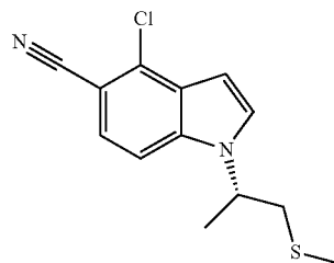
(S)-4-Chloro-1-(1-(methylthio)propan-2-yl)-1H-indole-5-carbonitrile
