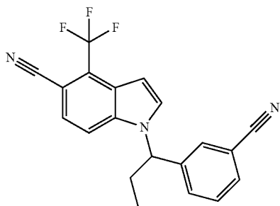
B. 1-(1-(3-Cyanophenyl)propyl)-4-(trifluoromethyl)-1H-indole-5-carbonitrile
