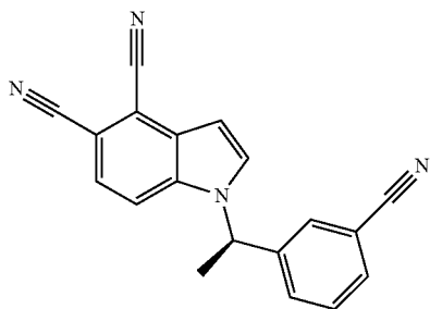
(R)-1-(1-(3-Cyanophenyl)ethyl)-1H-indole-4,5-dicarbonitrile
