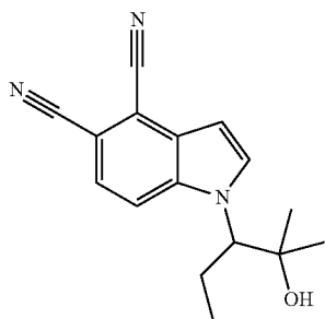
1-(2-Hydroxy-2-methylpentan-3-yl)-1H-indole-4,5-dicarbonitrile
