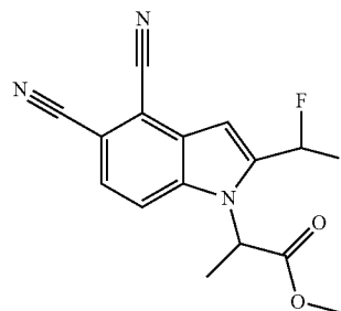
A. Methyl 2-(4,5-dicyano-2-(difluoromethyl)-1H-indol-1-yl)propanoate
