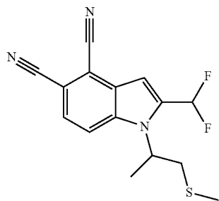
2-(Difluoromethyl)-1-(1-(methylthio)propan-2-yl)-1H-indole-4,5-dicarbonitrile
