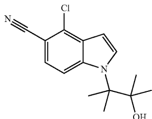
4-Chloro-1-(3-hydroxy-2,3-dimethylbutan-2-yl)-1H-indole-5-carbonitrile
