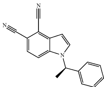
(R)-1-(1-Phenylethyl)-1H-indole-4,5-dicarbonitrile
