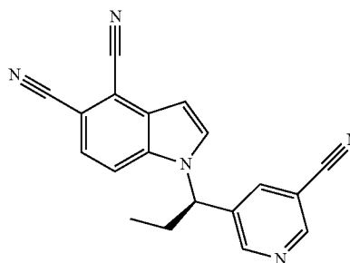
(R)-1-(1-(5-Cyanopyridin-3-yl)propyl)-1H-indole-4,5-dicarbonitrile
