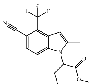
Methyl 2-[5-cyano-2-methyl-4-(trifluoromethyl)-1H-indol-1-yl]butanoate
