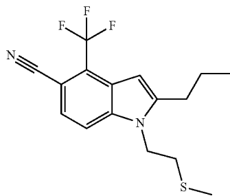
1-(2-(Methylthio)ethyl)-2-propyl-4-(trifluoromethyl)-1H-indole-5-carbonitrile
