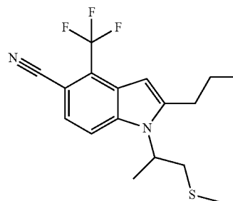
1-(1-(Methylthio)propan-2-yl)-2-propyl-4-(trifluoromethyl)-1H-indole-5-carbonitrile
