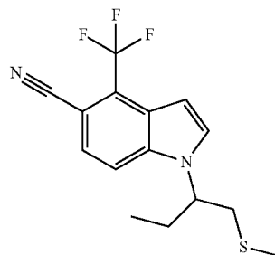
1-(1-(Methylthio)butan-2-yl)-4-(trifluoromethyl)-1H-indole-5-carbonitrile
