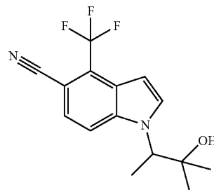
1-(3-Oxobutan-2-yl)-4-(trifluoromethyl)-1H-indole-5-carbonitrile (Ex. 19) and 1-(3-Hydroxy-3-methylbutan-2-yl)-4-(trifluoromethyl)-1H-indole-5-carbonitrile (Ex. 20)
