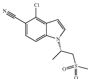
(S)-4-Chloro-1-(1-(methylsulfonyl)propan-2-yl)-1H-indole-5-carbonitrile
