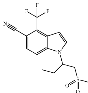
1-(1-(Methylsulfonyl)butan-2-yl)-4-(trifluoromethyl)-1H-indole-5-carbonitrile
