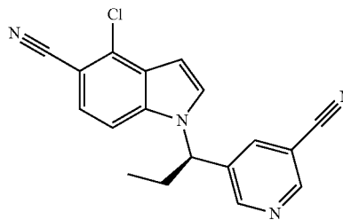
(R)-4-Chloro-1-(1-(5-cyanopyridin-3-yl)propyl)-1H-indole-5-carbonitrile
