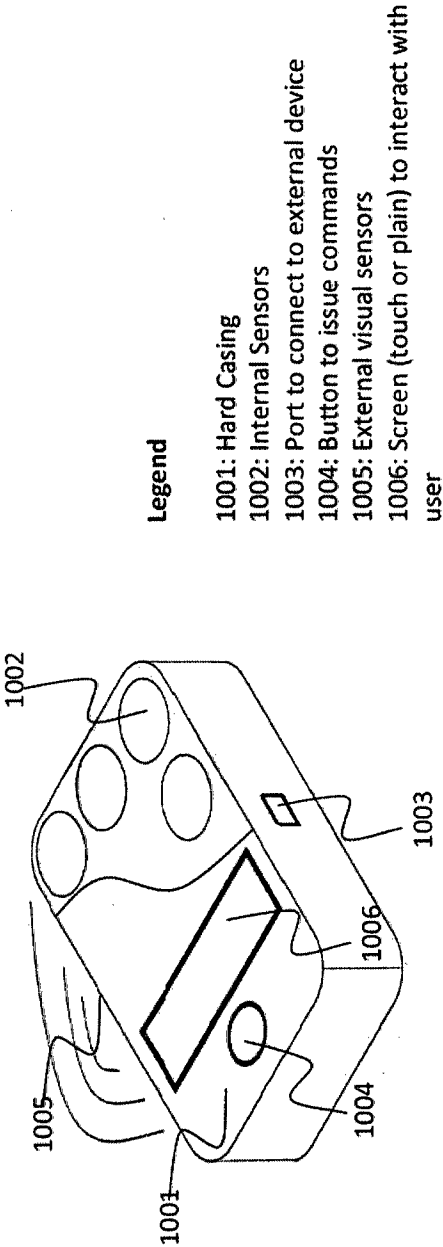
FIG 10 (1000): Sensor Device
