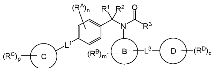
Formula (II)
