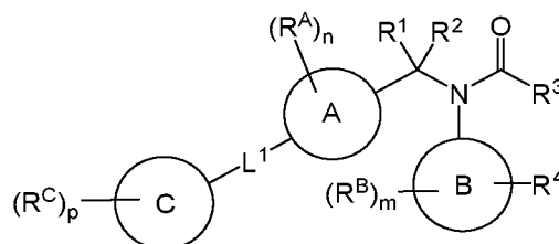
Formula (IV)
