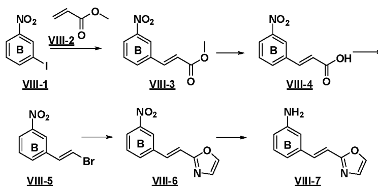
Scheme 8
