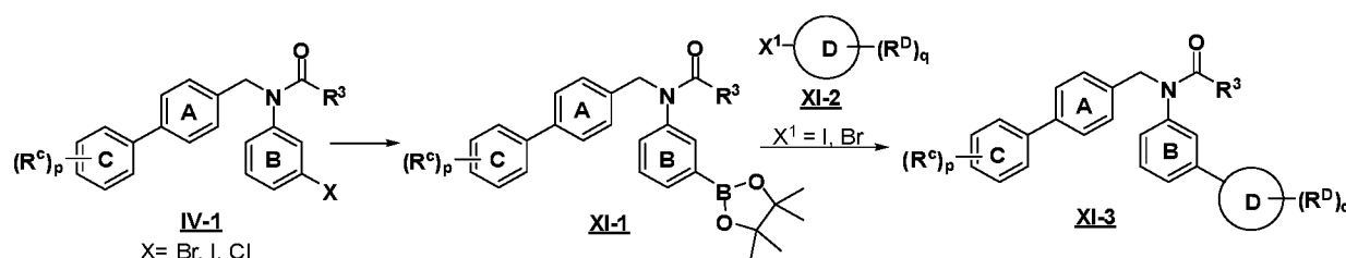
Scheme 11
