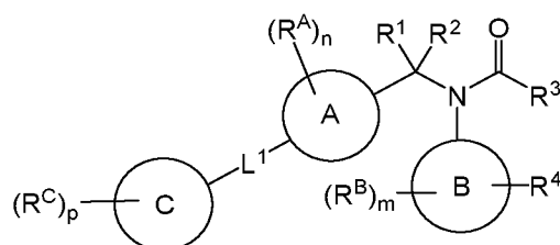
Formula (IV)
