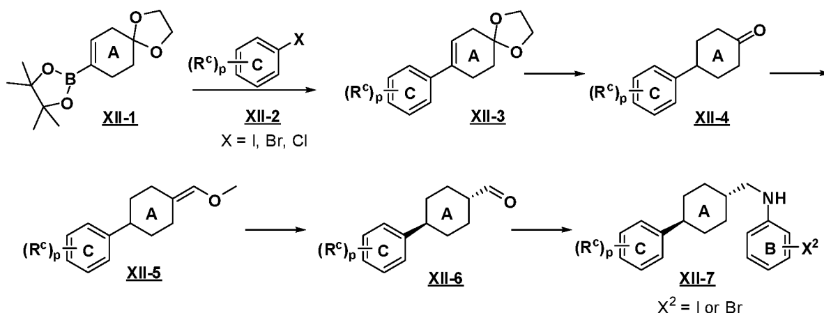
Scheme 12
