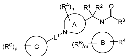
Formula (VI)
