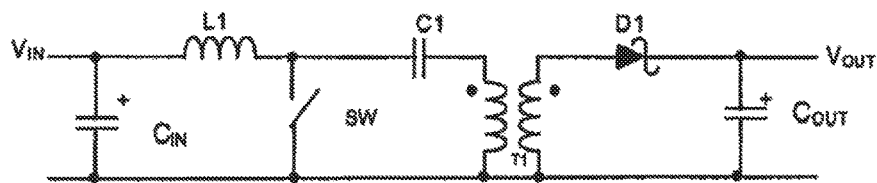
FIG. 20C (PRIOR ART)
