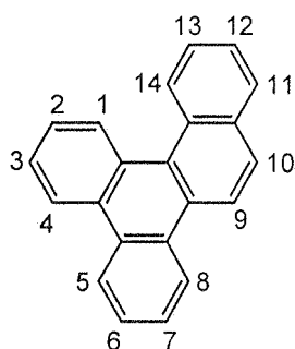
benzo[g]chrysene
