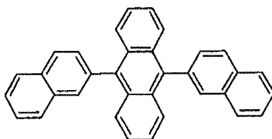
Compound B
