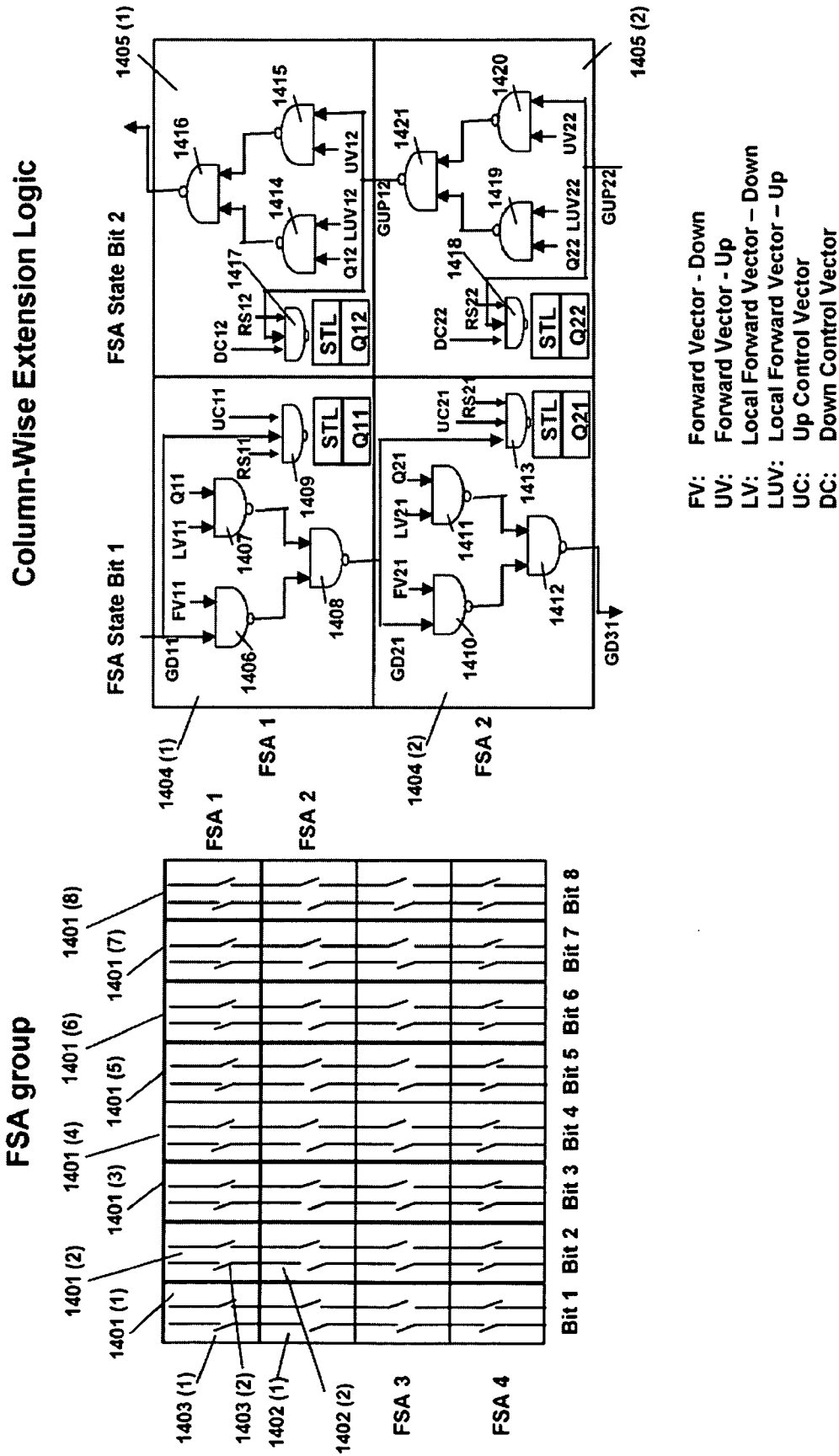
Fig. 14 PRISM Column-Wise FSA Extension
