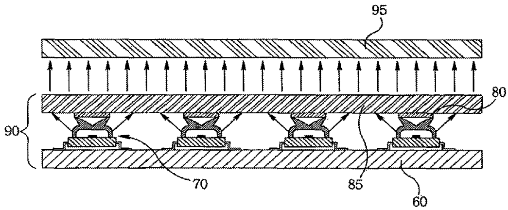
FIG. 6 (PRIOR ART)
