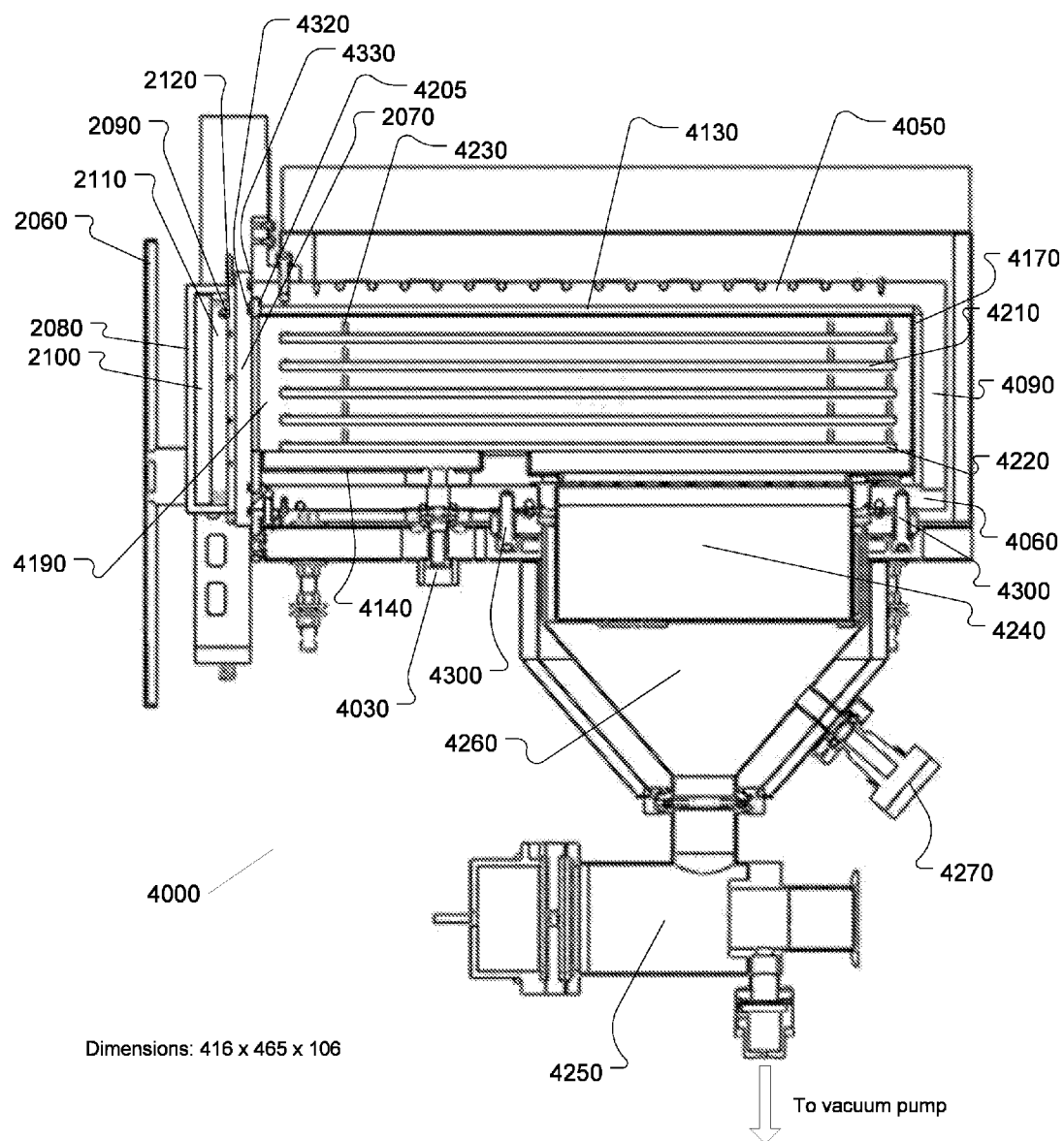
FIGURE 5 SIDE CUTAWAY VIEW
