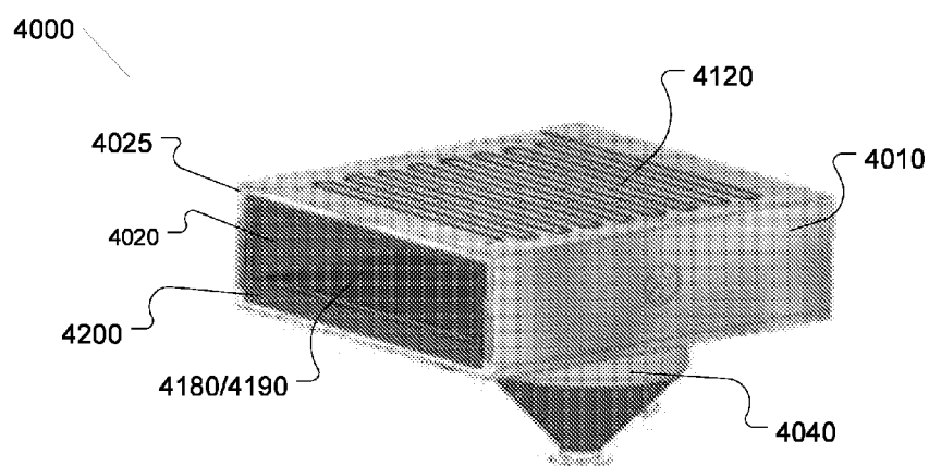
FIGURE 4 FIRST CHAMBER ASSEMBLY (ASSEMBLED)
