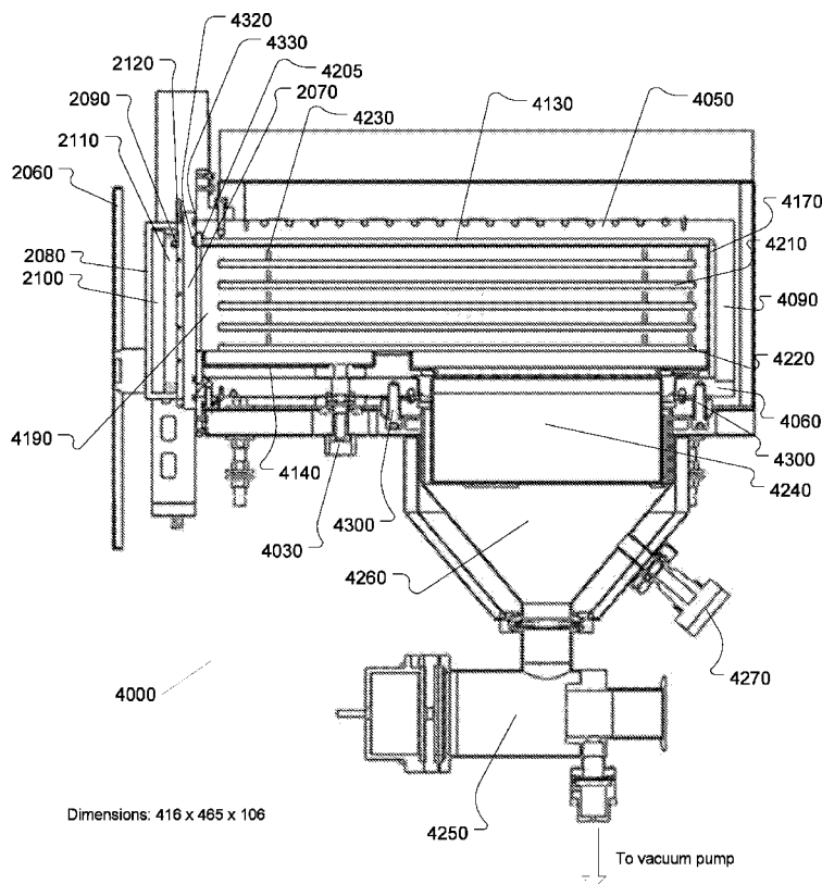
SIDE CUTAWAY VIEW
