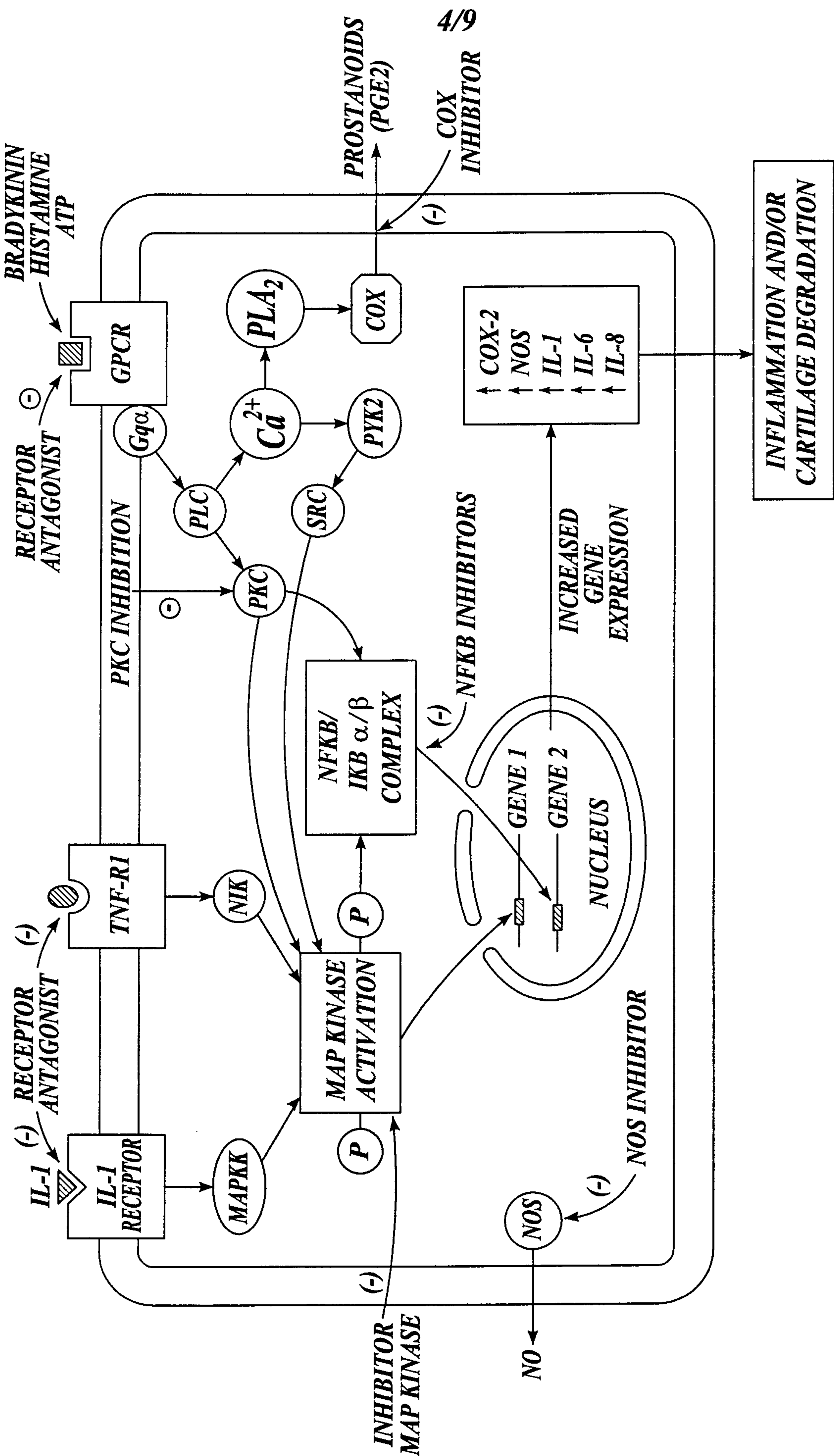
Fig. 4 MOLECULAR SITES OF ACTION IN CHONDROPROTECTIVE SOLUTION
