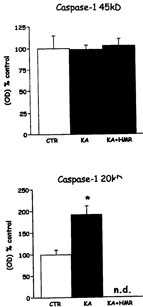
FIG. 1: Effect of compound 1 (25 \mu g in 4 \mu l icv) on caspase-1 levels (assessed by western blotting) in the hippocampus of kainic acid-treated rats. Rats were killed 90 min after the beginning of EEG seizures induced by intrahippocampal application of 40 ng kainic acid.
