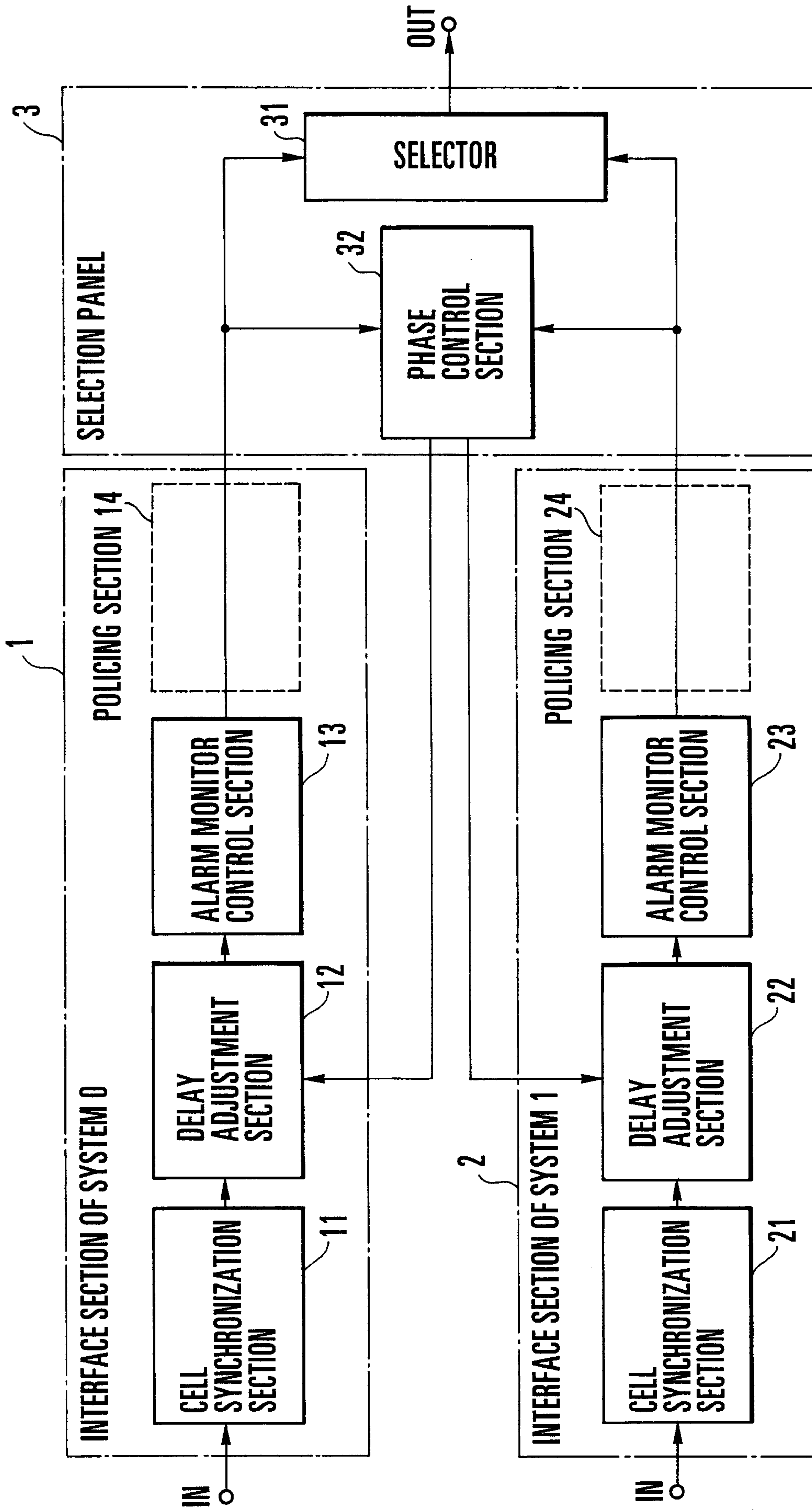
FIG. 2 PRIOR ART
