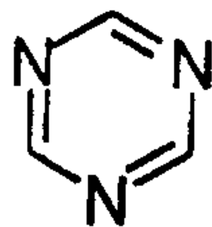
triazine (triazinyl)
