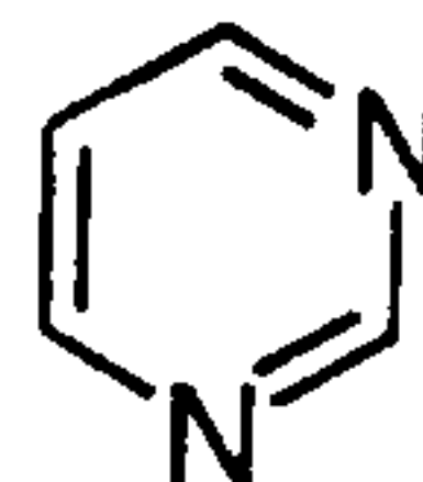
pyrimidine (pyrimidinyl)
