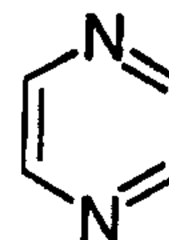
pyrazine (pyrazinyl)
