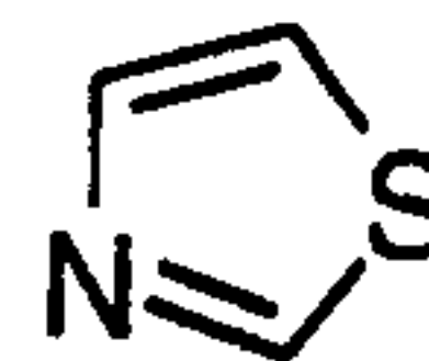
thiazole (thiazolyl)
