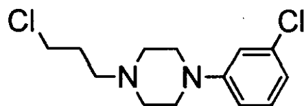
Compound-II free base
