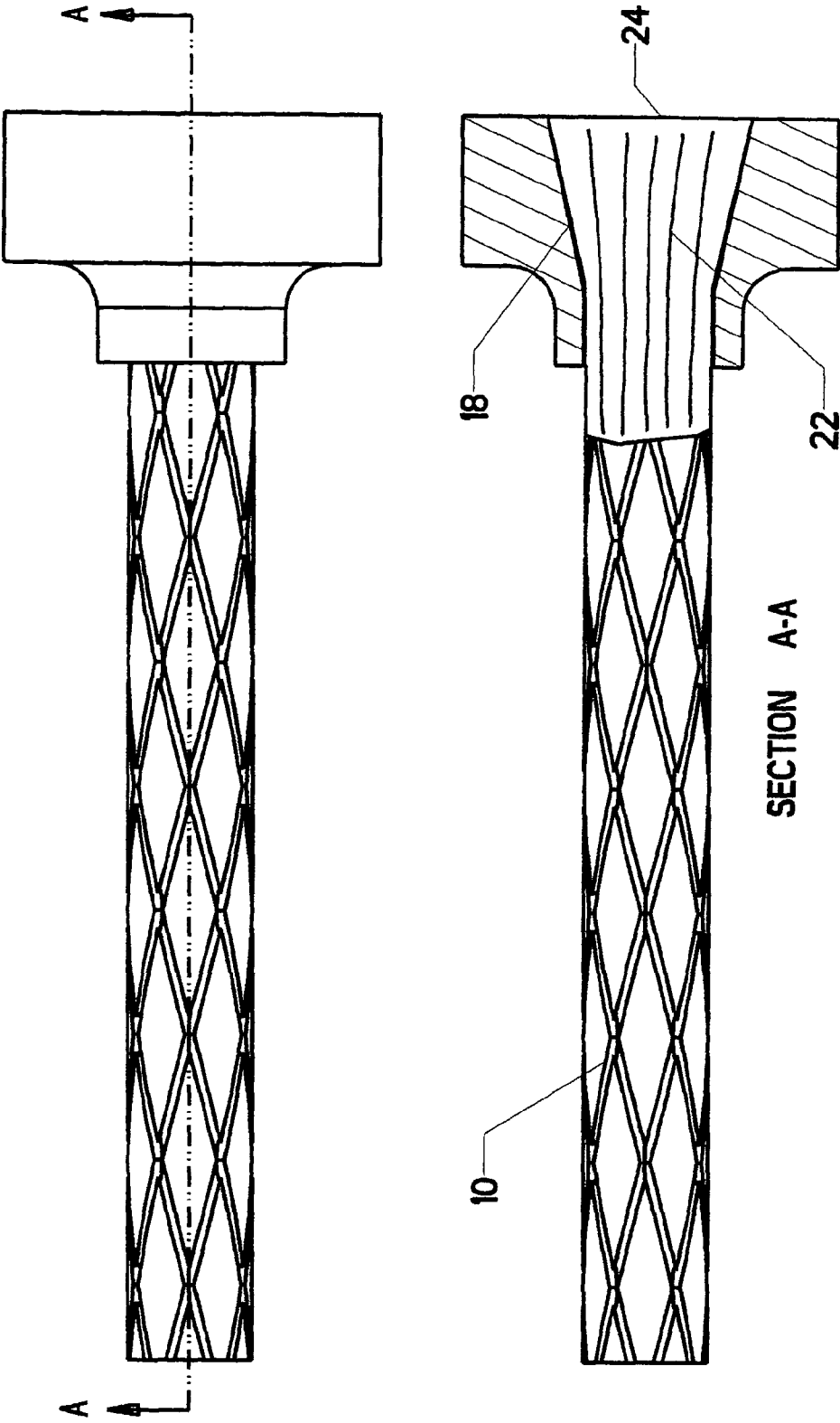
FIG. 3 (PRIOR ART)
