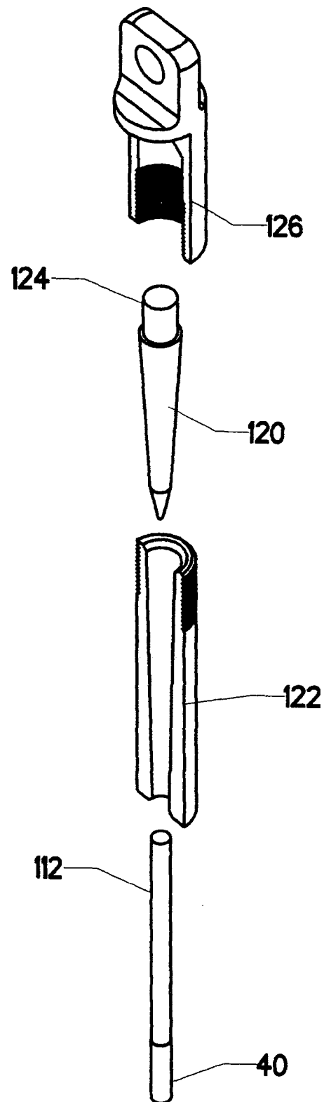
FIG 36 (PRIOR ART)
