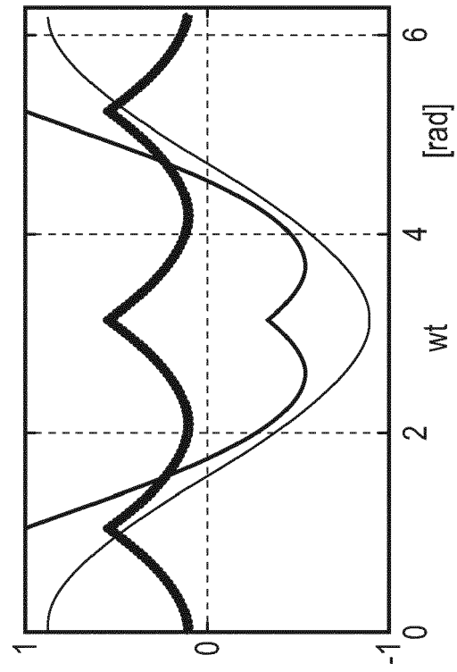
(a) Equation (2)
