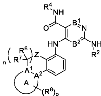
Formula (IV)
