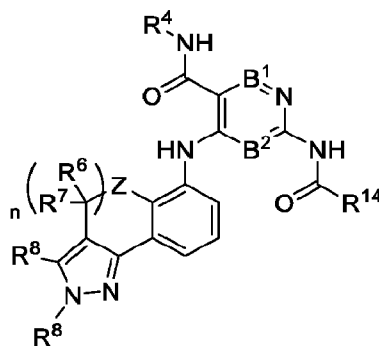
Formula (IXa-1)
