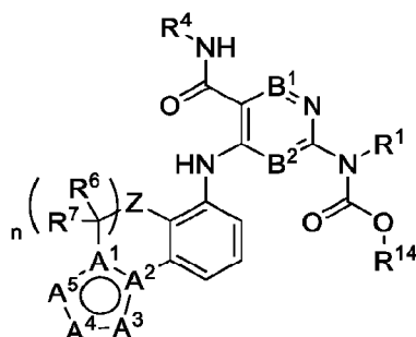
Formula (XI)
