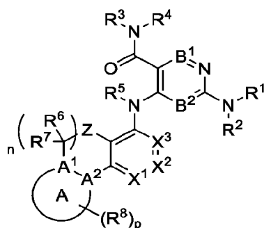
Formula (Ia)
