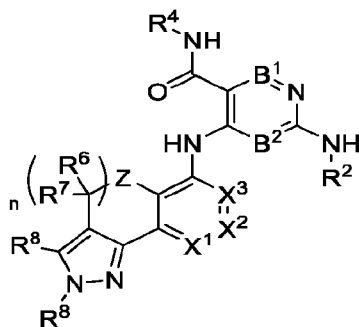
Formula (XVII)
