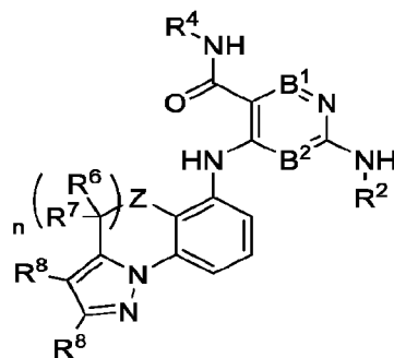
Formula (VI-f-1)
