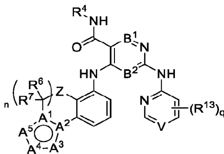
Formula (VIII)
