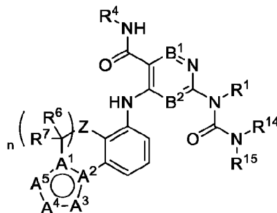
Formula (X)
