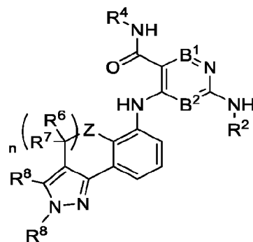
Formula (VIa-1)
