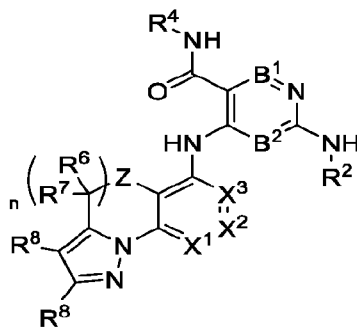
Formula (XVIII)
