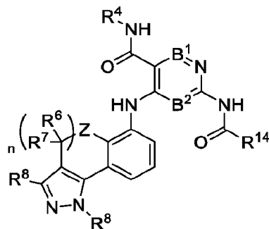
Formula (IXc-1)
