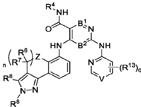
Formula (VIIIa-1)
