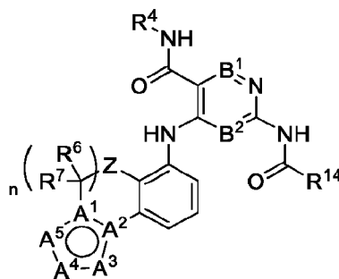
Formula (IX)
