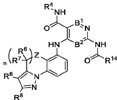
Formula (IXf-1)
