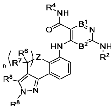
Formula (VIa-1)
