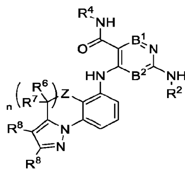
Formula (VIf-1)
