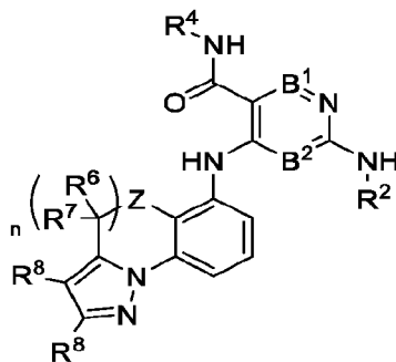
Formula (VIf-1)
