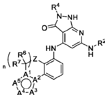
Formula (XII)
