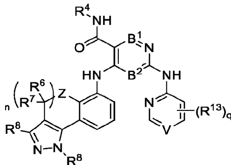
Formula (VIIIc-1)
