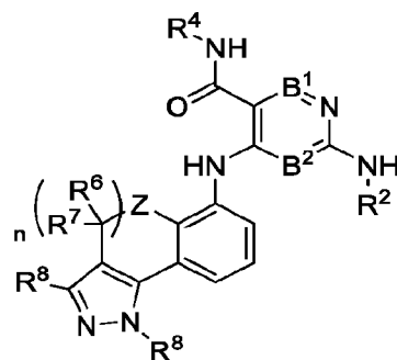
Formula (VIc-1)
