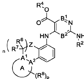
Formula (V)
