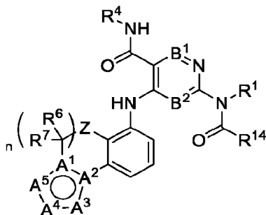
Formula (IX)
