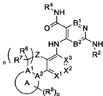
Formula (II)
