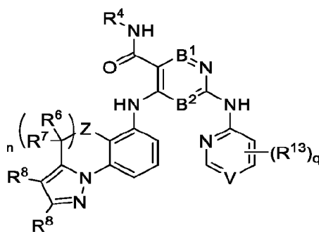
Formula (VIIIf-1)
