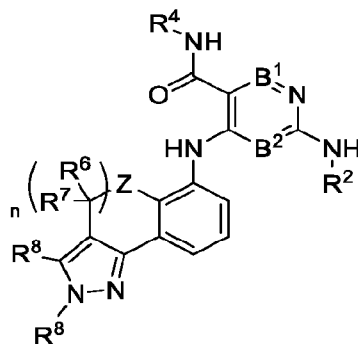
Formula (VIa-1)
