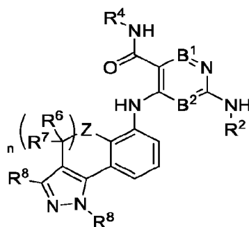
Formula (VIc-1)
