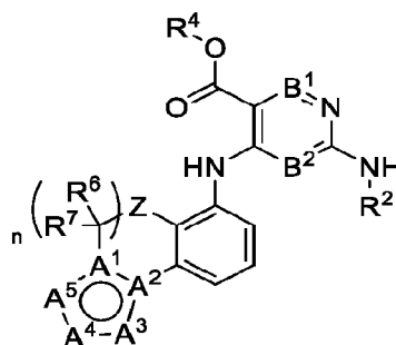
Formula (VII)
