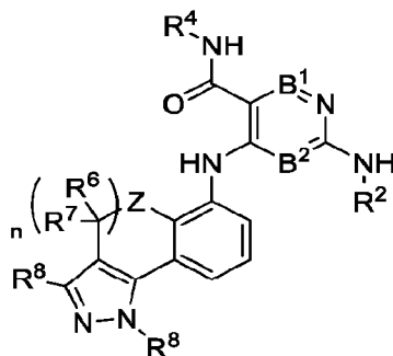
Formula (VIc-1)
