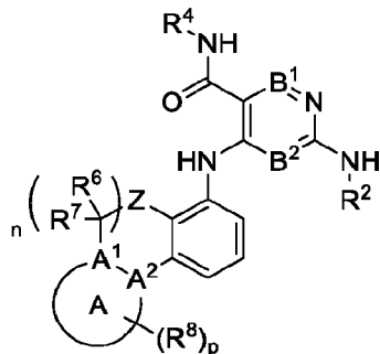
Formula (IV)
