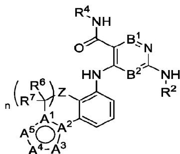
Formula (VI)
