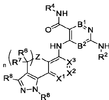
Formula (XV)
