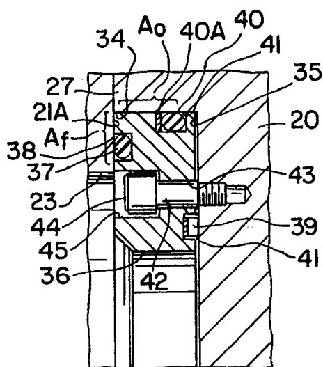
FIG. 3 (PRIOR ART)
