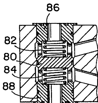
FIG. 10 (PRIOR ART)
