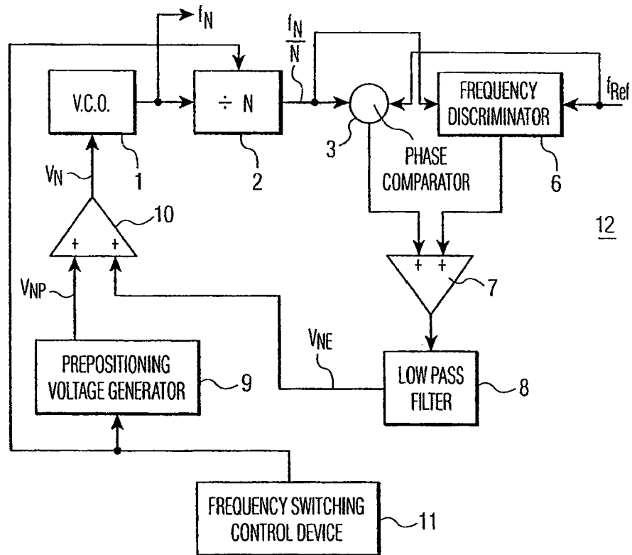
FIG. 2 PRIOR ART
