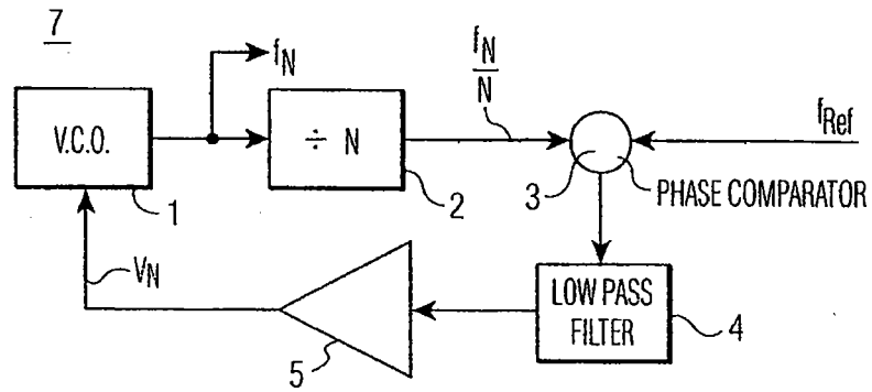
FIG. 1 PRIOR ART
