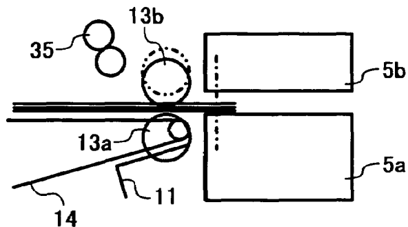
FIG. 9C STAPLER MOVEMENT
