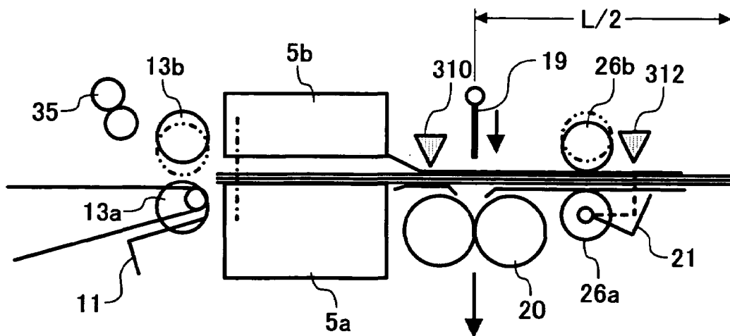
FIG. 10D FOLDING
