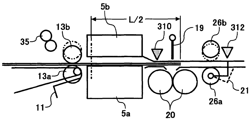
FIG. 10B BUNDLE FEED → BINDING
