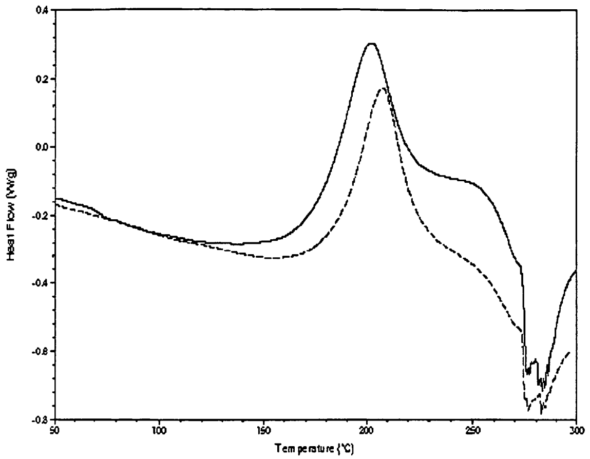
Figure 4: DSC-diagram
