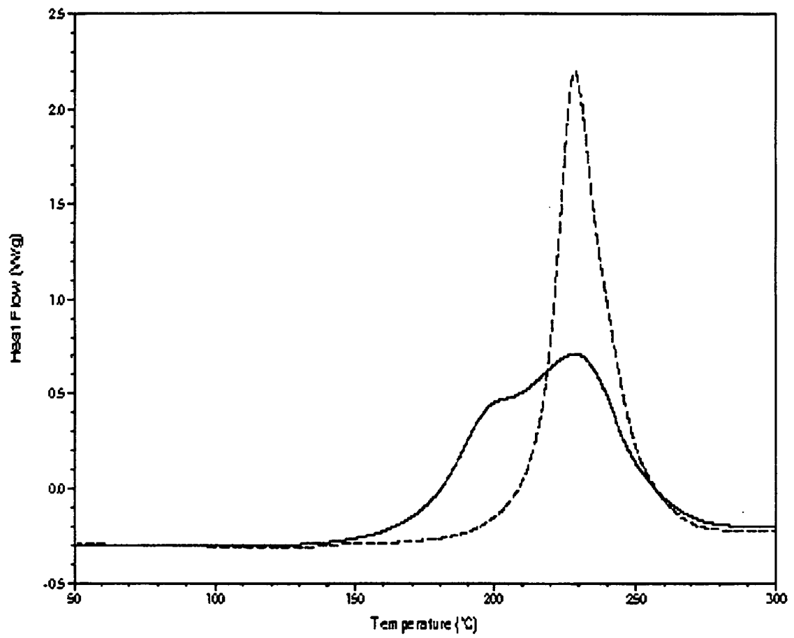
Figure 3: DSC-diagram
