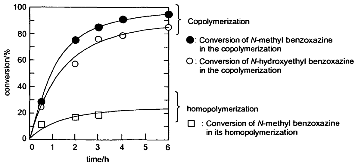
Figure 2: Time conversion relationships
