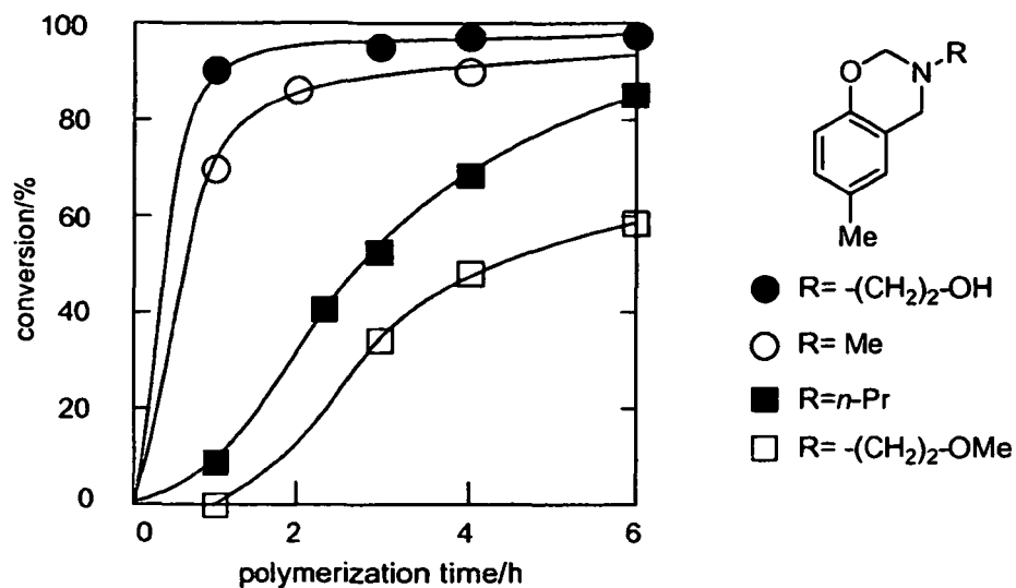
Figure 1: Time-conversion relationships for the polymerization of different benzoxazines
