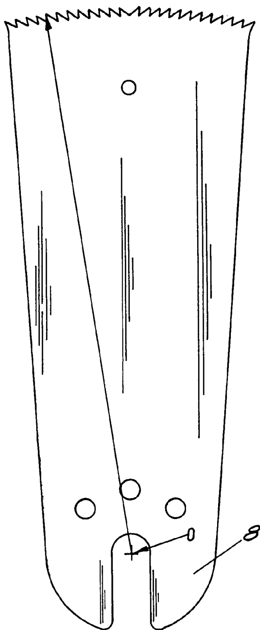
PRIOR ART Fig 6A
