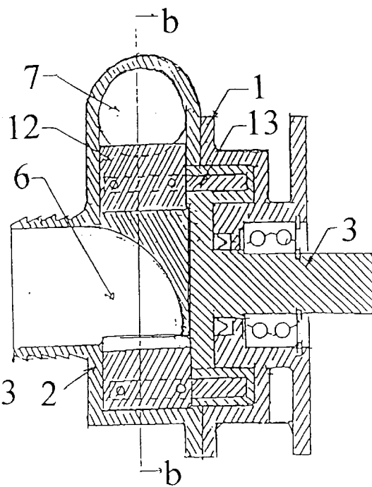
FIG 3B section aa
