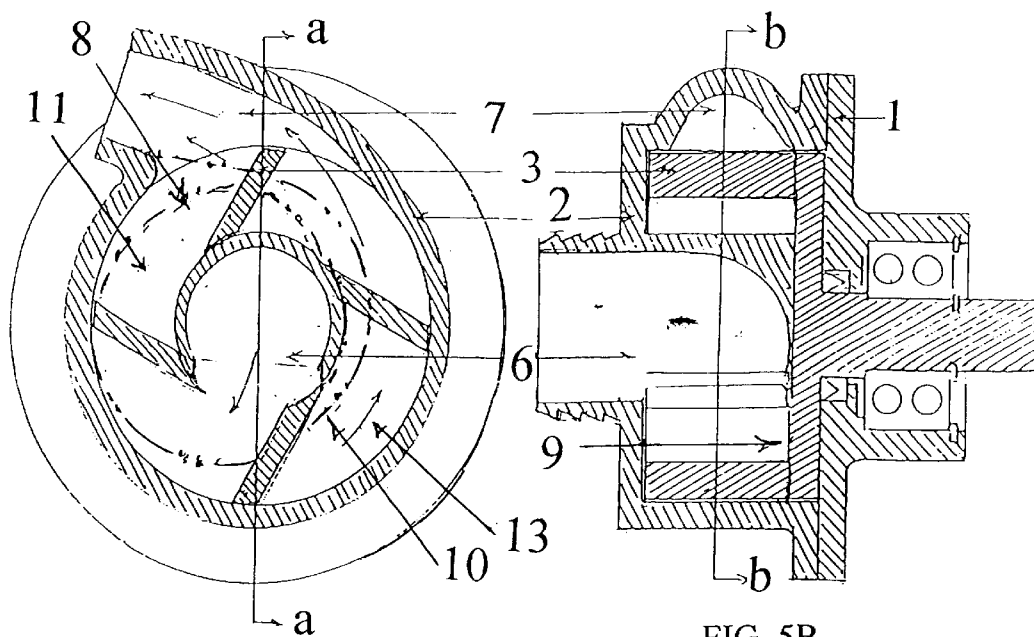
FIG 5A section bb
