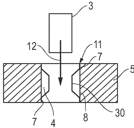
FIG. 3 (Prior Art)
