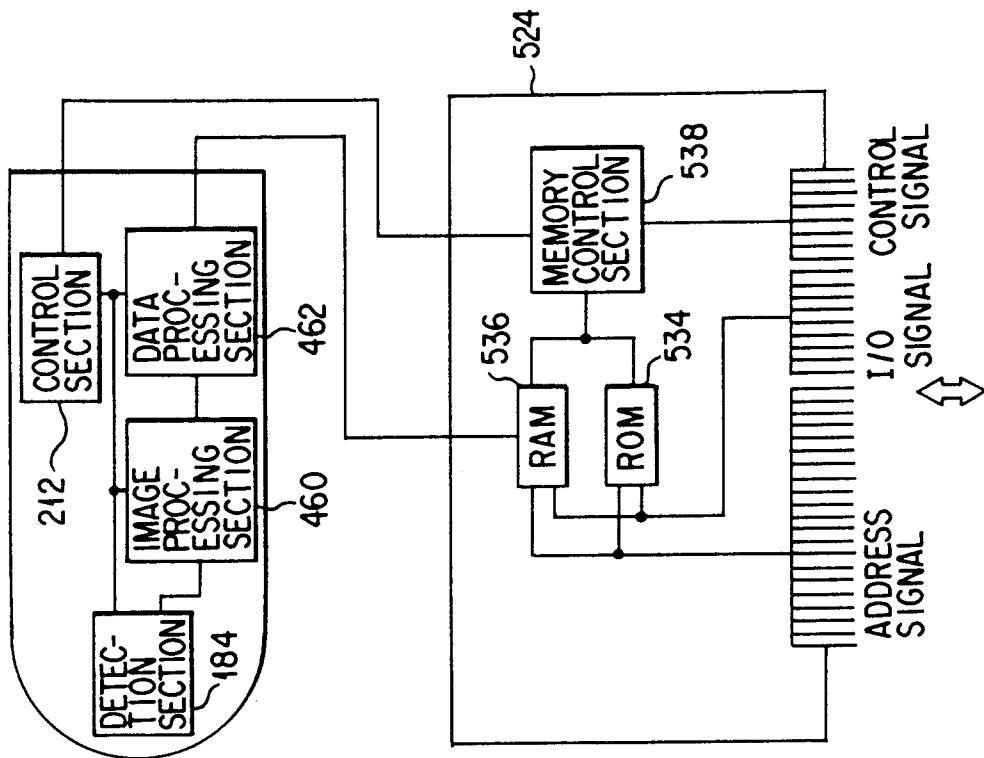
VIDEO GAME APPARATUS BODY FIG. 71
