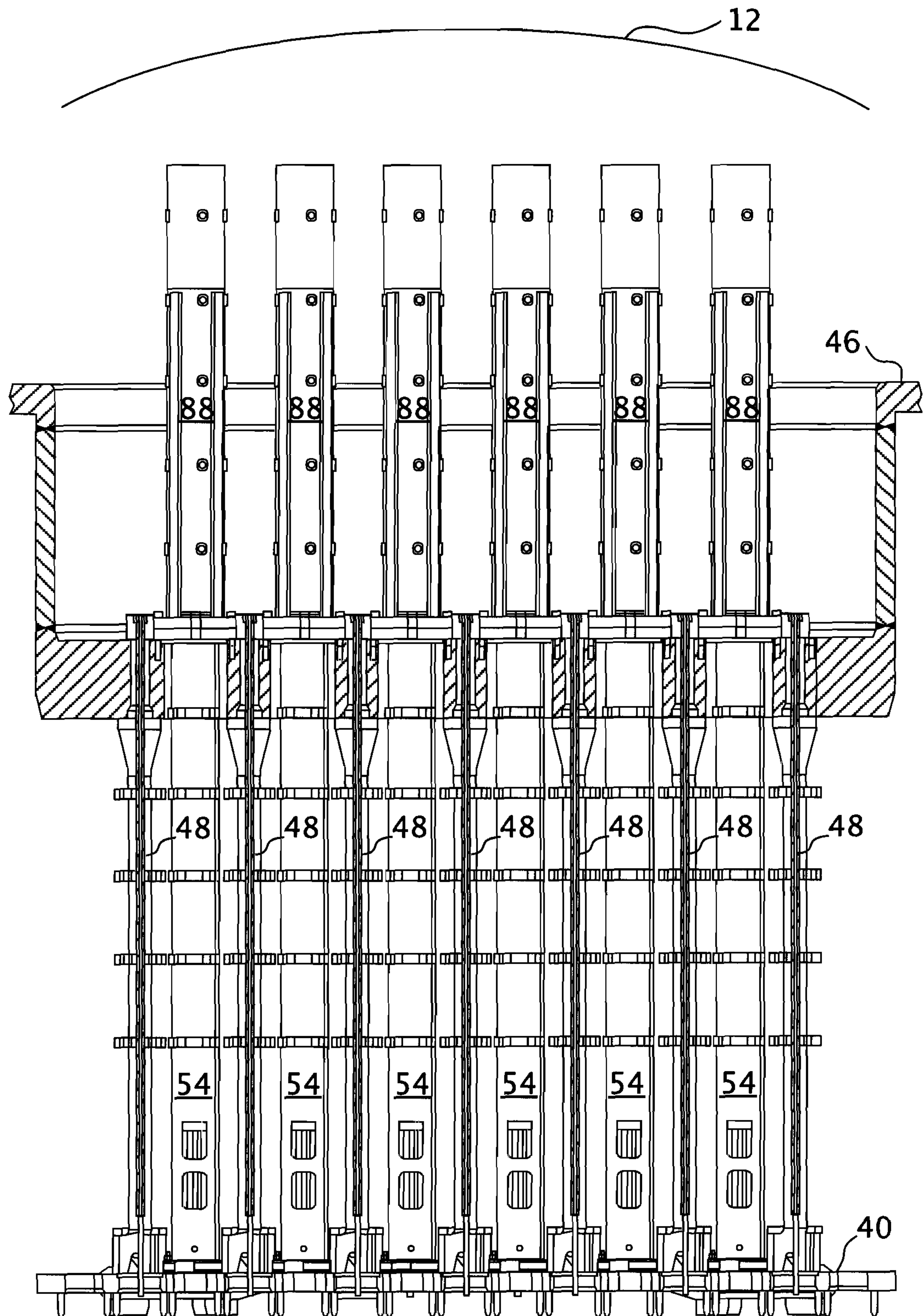
FIG. 3 Prior Art
