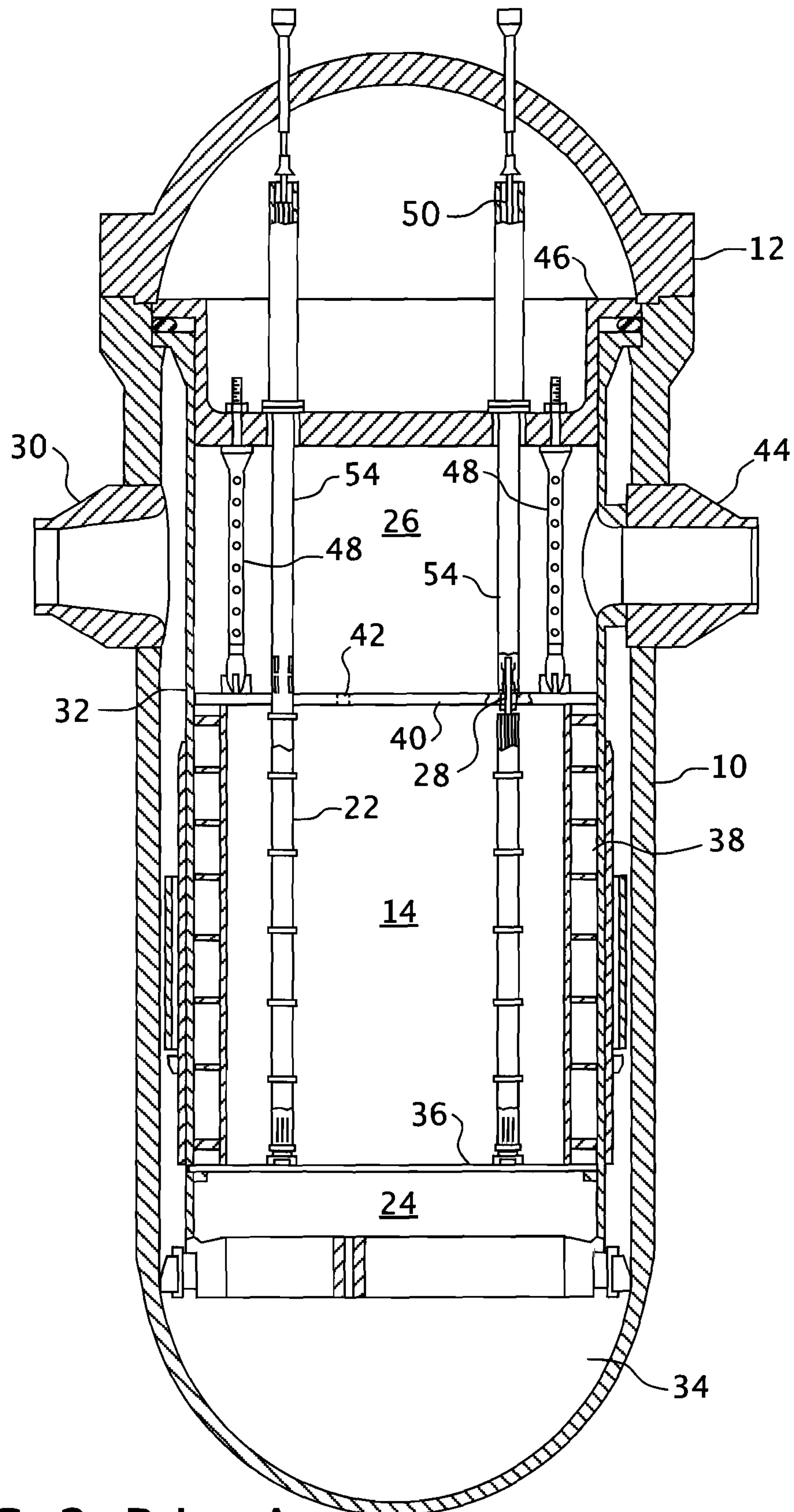
FIG. 2 Prior Art
