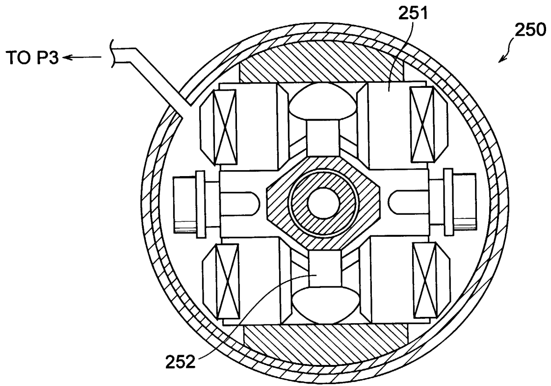
B-B SECTION
