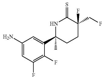
(3R,6S)-6-(5-amino-2,3-difluorophenyl)-3-fluoro-3-(fluoromethyl)-6-methylpiperidine-2-thione and
