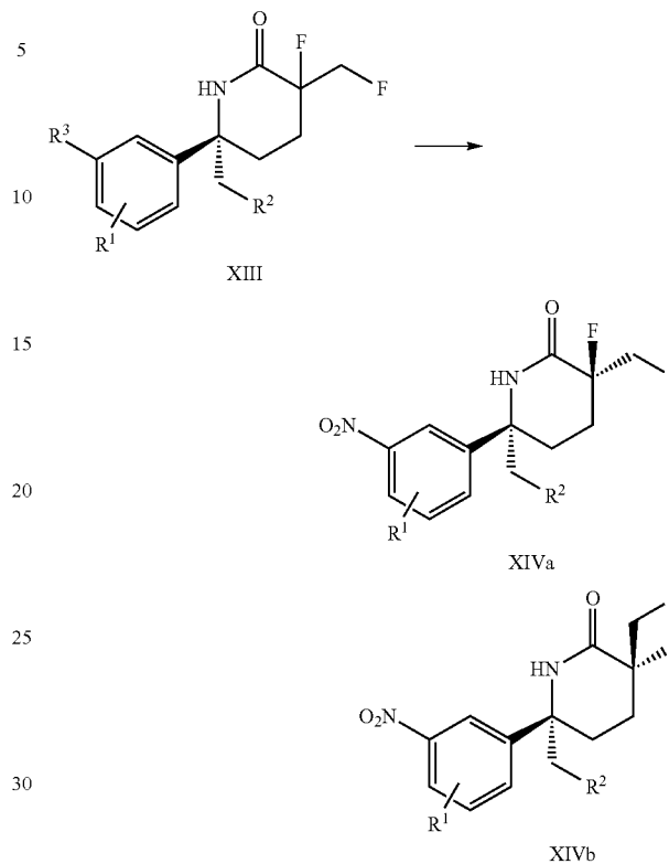
Scheme 3
