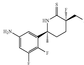
(3S,6S)-6-(5-amino-2,2-difluorophenyl)-3-fluoro-3-(fluoromethyl)-6-methylpiperidine-2-thione;
