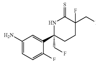
(6S)-6-(5-amino-2-fluorophenyl)-3-fluoro-3,6-bis(fluoromethyl)piperidine-2-thione.
