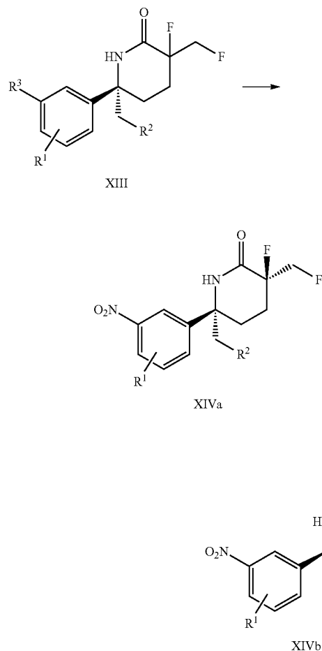
Scheme 2
