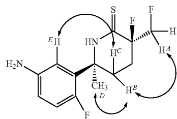
Scheme 6. nOe in ROESY of (3 R ,6 S )-6-(5-amino-2-fluorophenyl)-3-fluoro-3-(fluoromethyl)-6-methylpiperidine-2-thione
