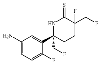
(6S)-6-(5-amino-2-fluorophenyl)-3-fluoro-3,6-bis(fluoromethyl)piperidine-2-thione, and salts thereof.
