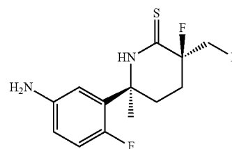
(3R,6S)-6-(5-amino-2-fluorophenyl)-3-fluoro-3-(fluoromethyl)-6-methylpiperidine-2-thione;
