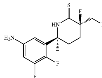
(3R,6S)-6-(5-amino-2,3-difluorophenyl)-3-fluoro-3-(fluoromethyl)-6-methylpiperidine-2-thione; and
