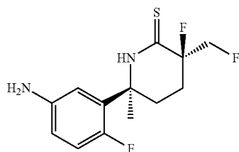
(3R,6S)-6-(5-amino-2-fluorophenyl)-3-fluoro-3-(fluoromethyl)-6-methylpiperidine-2-thione
