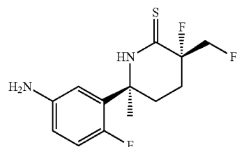
(3S,6S)-6-(5-amino-2-fluorophenyl)-3-fluoro-3-(fluoromethyl)-6-methylpiperidine-2-thione;
