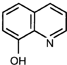
8-Hydroxyquinoline
