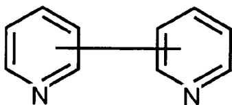
bipyridines
