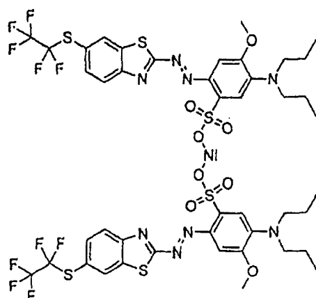
Compound C
