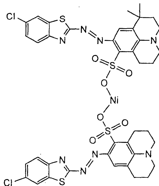
Compound H
