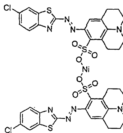
Compound G
