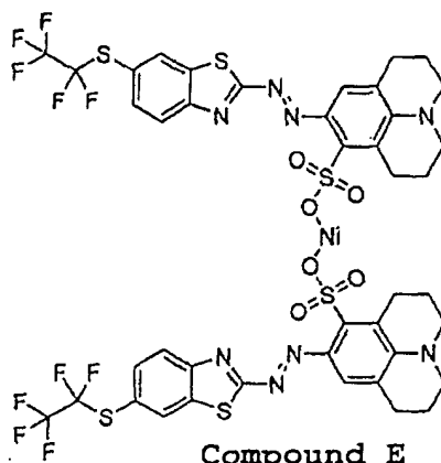
Compound E
