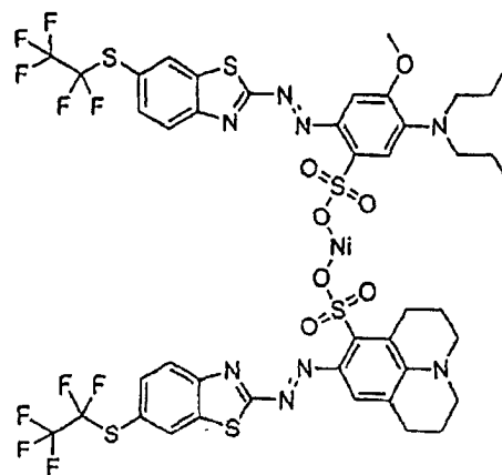
Compound D
