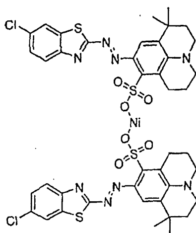
Compound F
