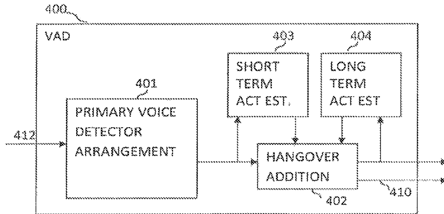
FIGURE 4B
