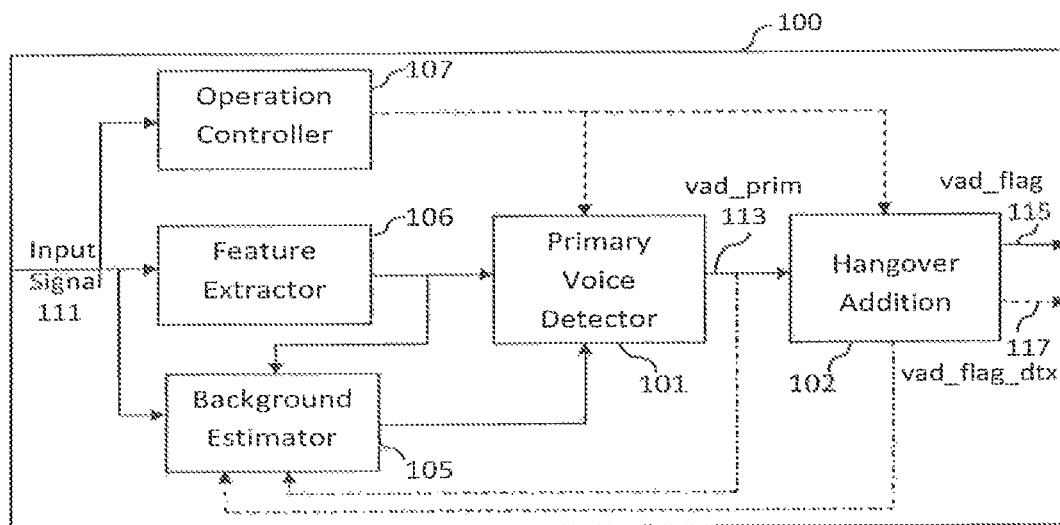
FIGURE 1 (Prior Art)
