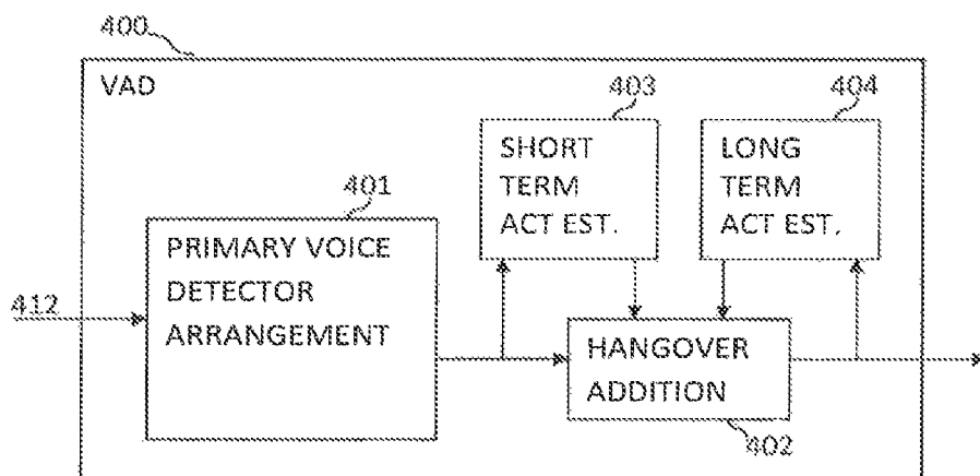
FIGURE 4A
