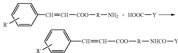
Reaction scheme (3)
