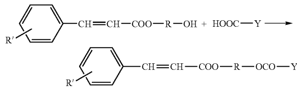
Reaction scheme (4)
