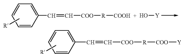
Reaction scheme (1)
