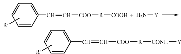
Reaction scheme (2)
