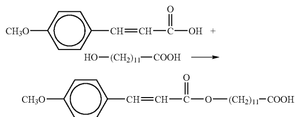
Reaction scheme (8)
