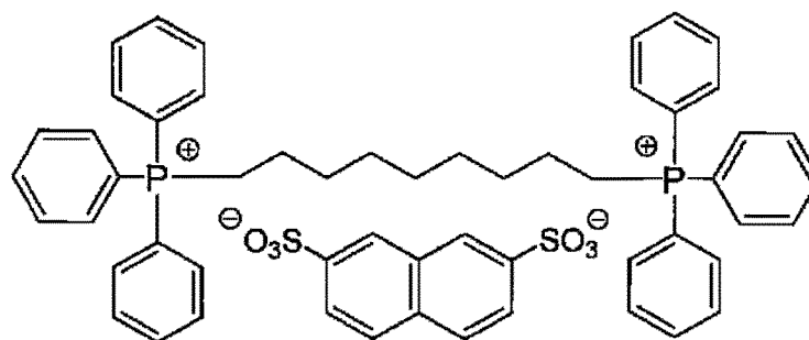
Additive 1
