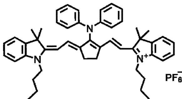
Infrared absorbent 4
