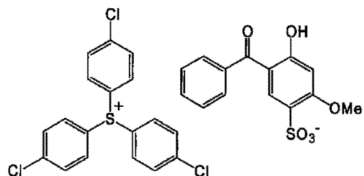
Polymerization initiator 2
