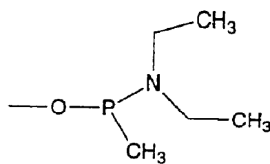
N,N-diethylamino-methyl- phosphine
