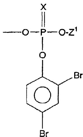
2,4-dibromophenyl phosphate
