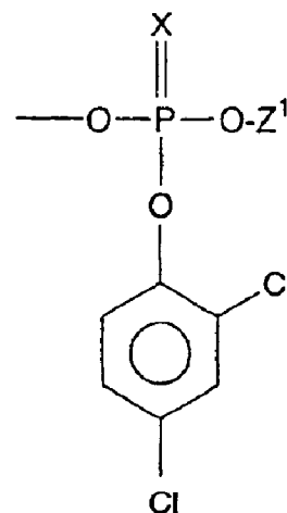
2,4-dichlorophenyl phosphate
