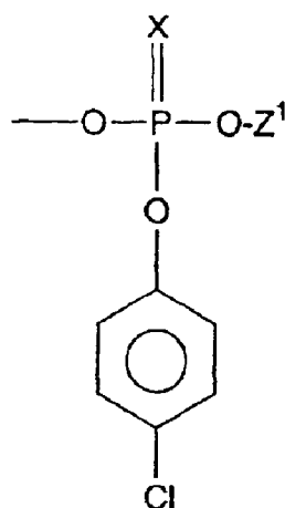
4-chlorophenyl phosphate
