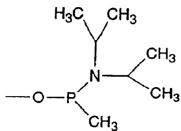
N,N-diisopropylamino-methyl- phosphine
