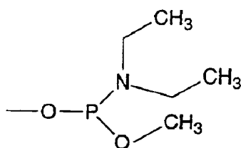
N,N-diethylamino-methoxyphosphine
